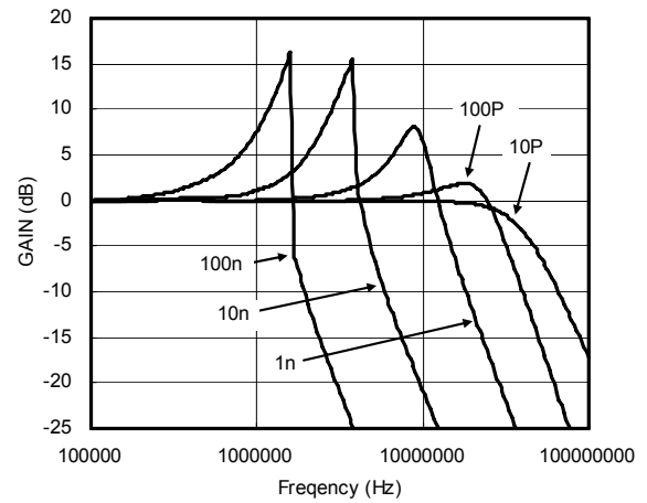
Frequency Response vs. Various C_L
