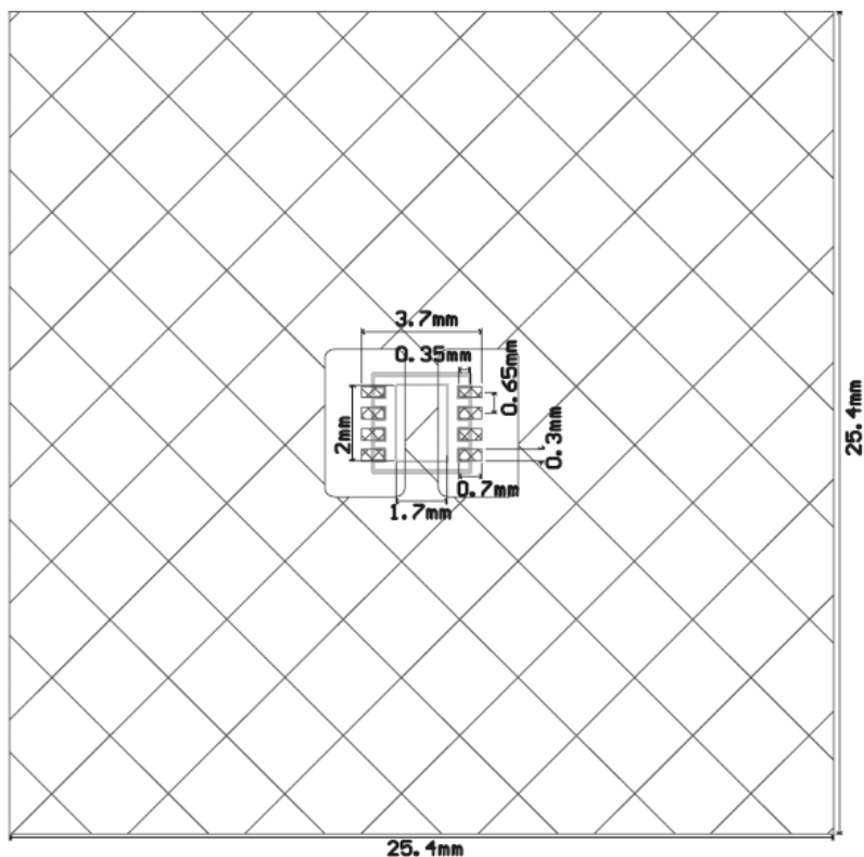
MSOP-8 (FD)
