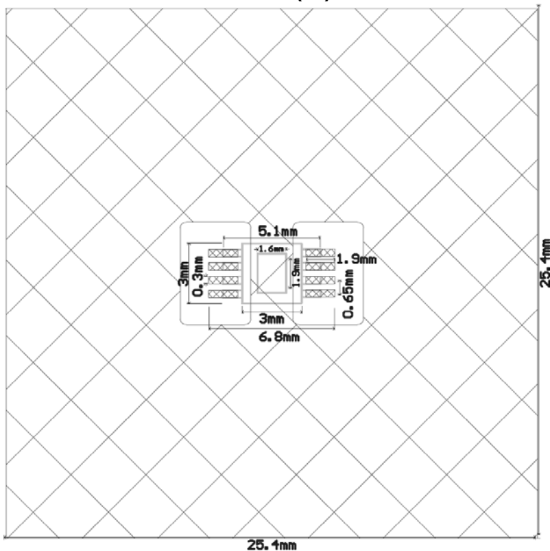
MSOP-8 (FD)
