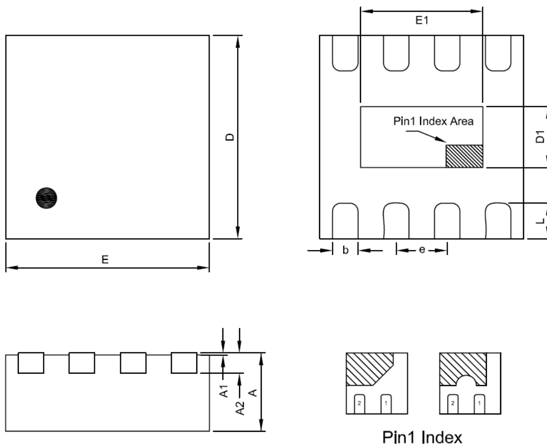
TDFN2X2-8 Package
