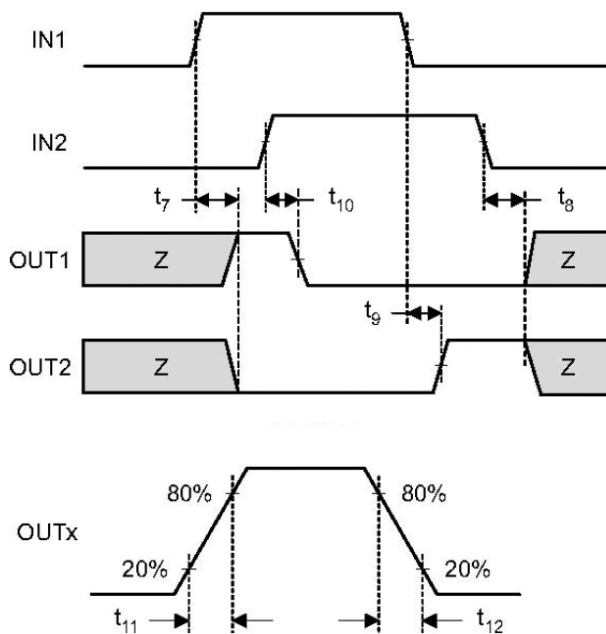
Figure 2. Input and Output Timing for G2056
