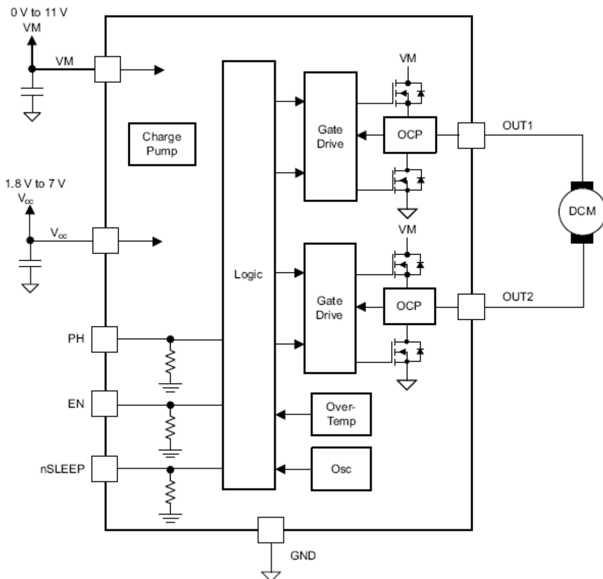
Figure 9. G2056A Functional Block Diagram
