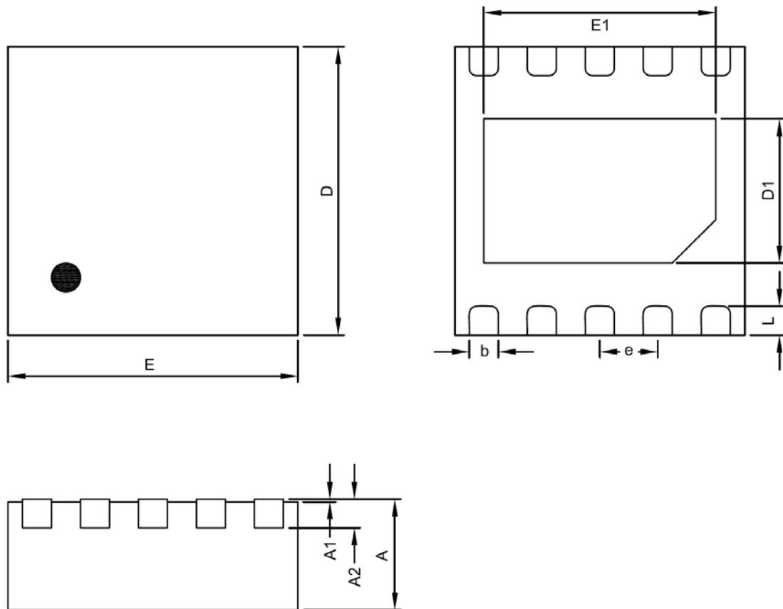
TDFN2X2-10 Package
