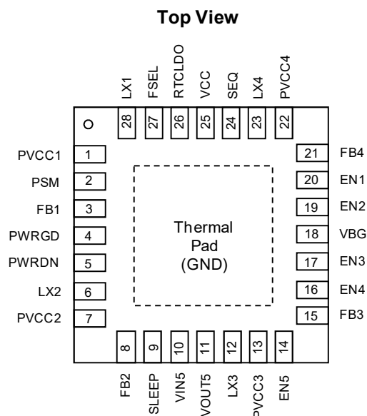
G2225 TQFN4X4-28
