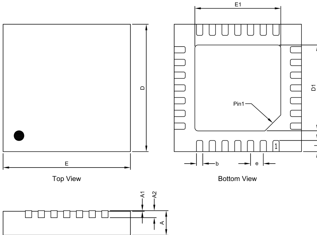
TQFN4X4-28 Package
