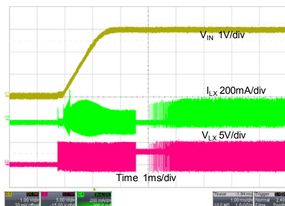
CH3 VIN=3.6V, Vout=3V, Iout=30mA (PSM)
