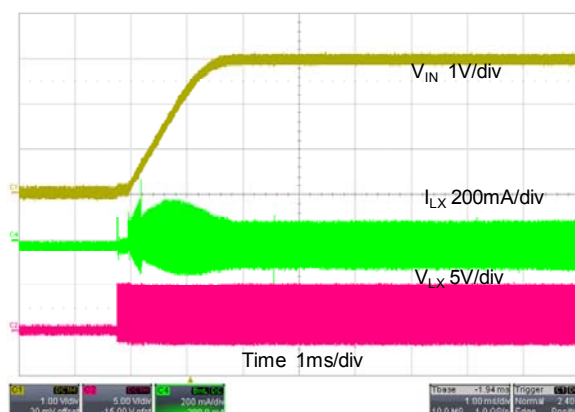
CH3 VIN=3.6V, Vout=3V, NO load (PWM)
