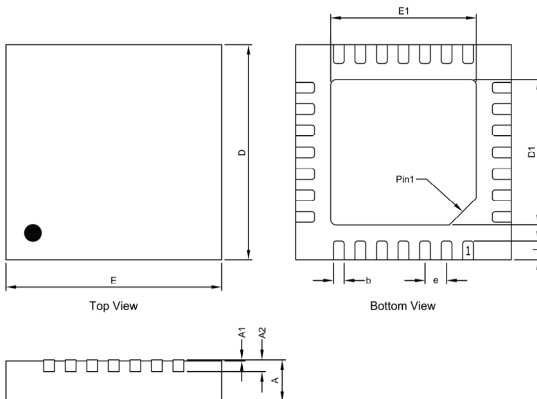
TQFN4X4-28 Package
