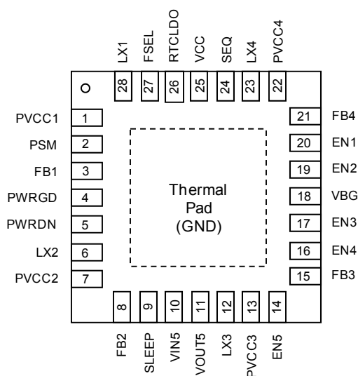
G2253 TQFN4X4-28
