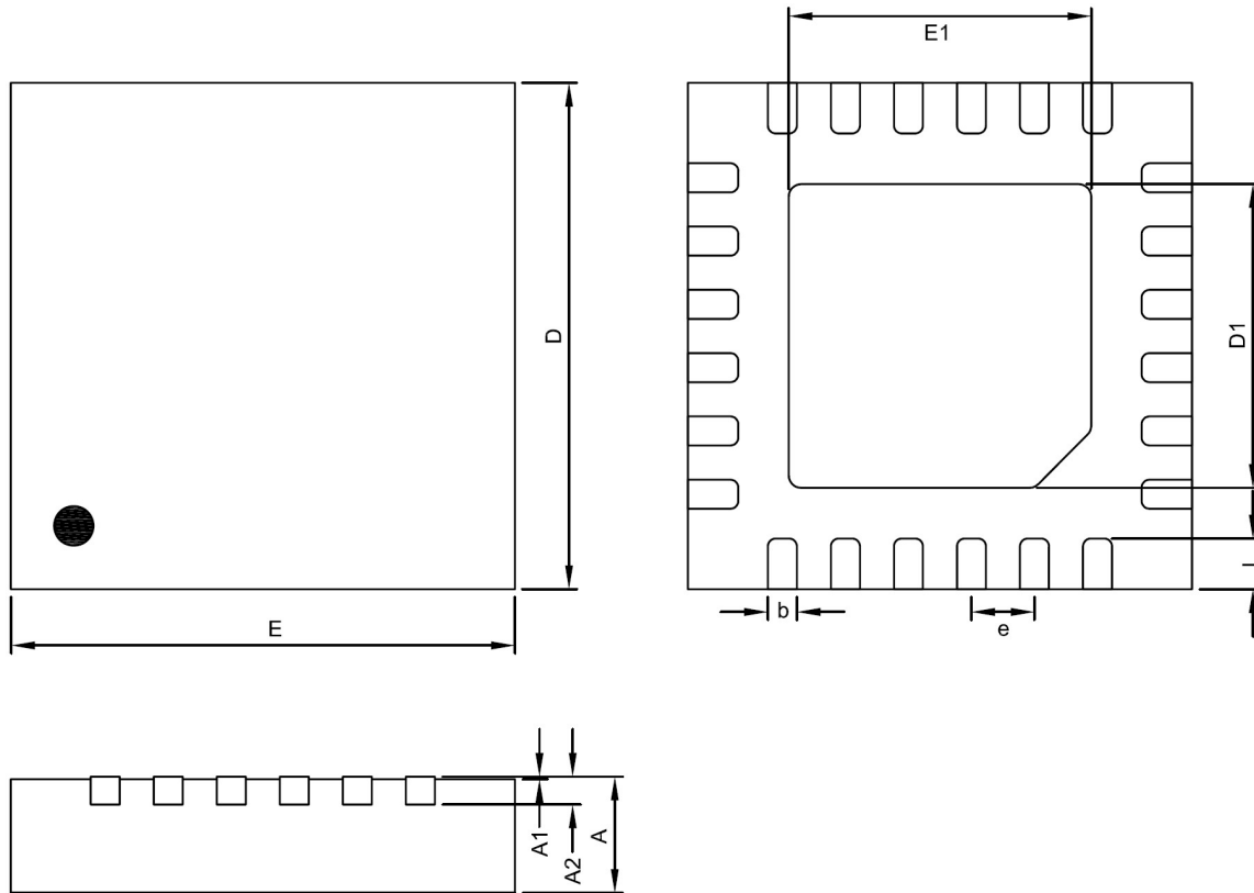
QFN4X4-24 Package
