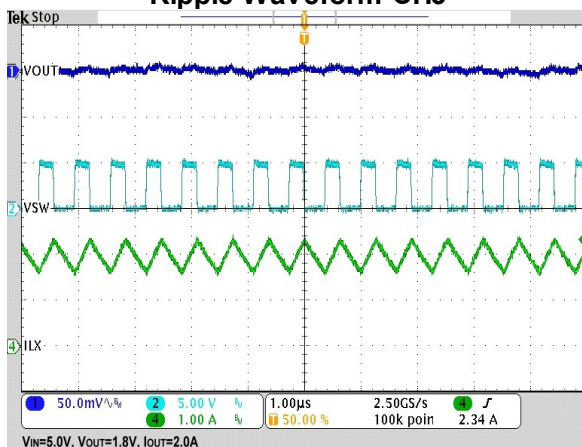
Ripple Waveform-CH3
