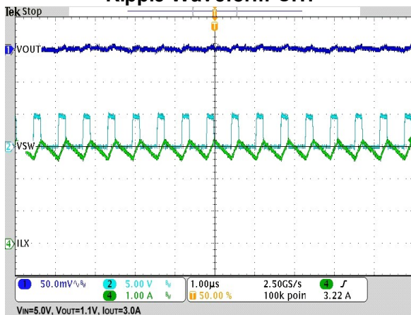
Ripple Waveform-CH1
