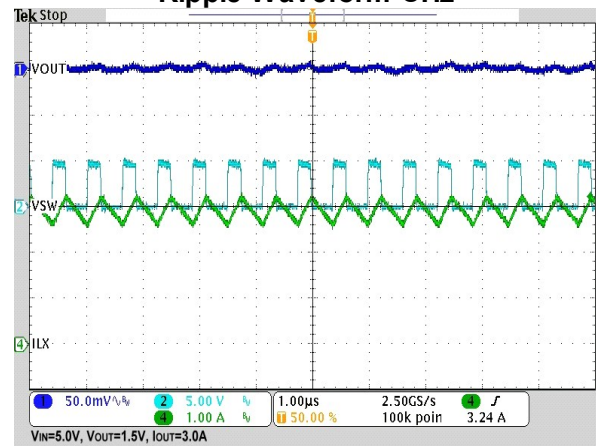
Ripple Waveform-CH2
