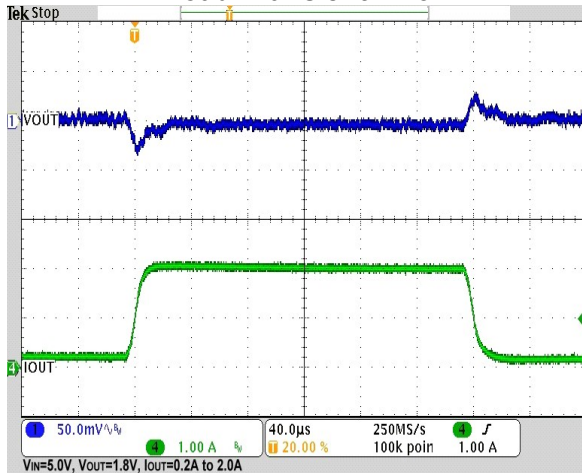
Load Transient-CH3
