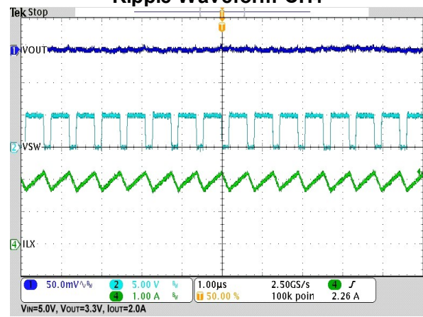
Ripple Waveform-CH4
