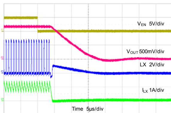
Start-down Through Enable V_{OUT}=1.2V , I_{OUT}=1A
