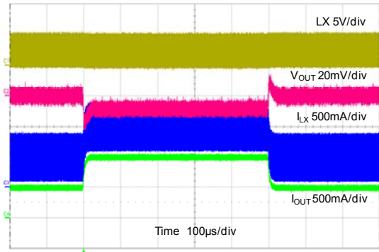
Load Transient Response V_{OUT}=1.2V, I_{OUT}=500mA \sim 1A
