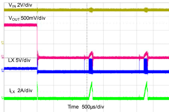
Short Circuit waveform V_{OUT}=1.2V
