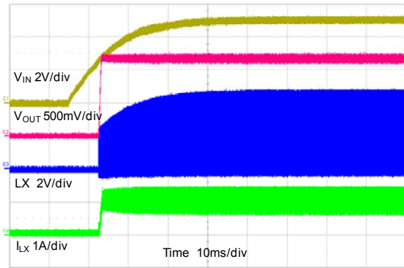
Start-up Through VIN V_{OUT}=1.2V, I_{OUT}=1A
