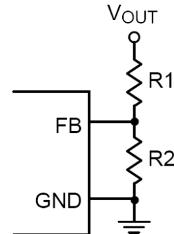
Figure 1. Setting V_{OUT} with a Voltage Divider
