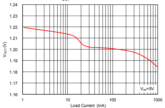
V_{OUT} vs. Load Current
