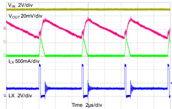
V_{OUT}=1.2V , I_{OUT}=50mA
