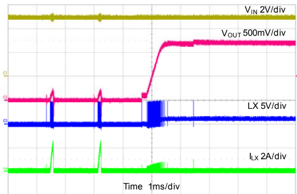
Short Circuit Recovery V_{OUT}=1.2V
