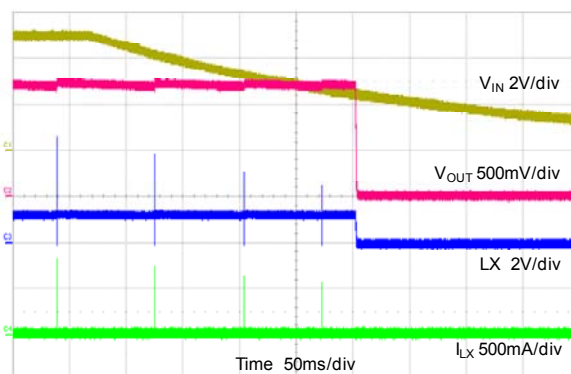
Start-down Through VIN V_{OUT}=1.2V , No Load
