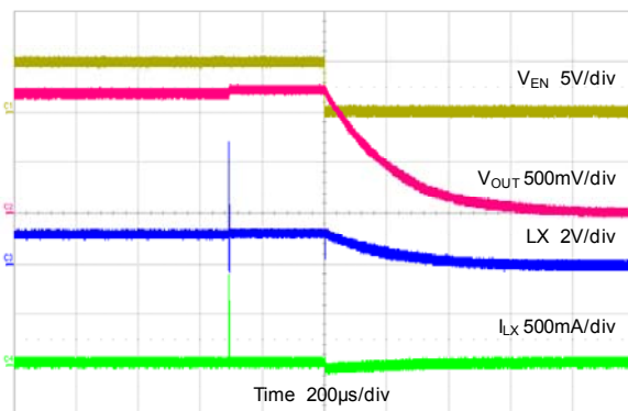
Start-down Through Enable V_{OUT}=1.2V , No Load
