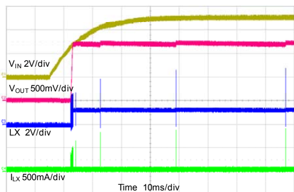
Start-up Through VIN V_{OUT}=1.2V , No Load
