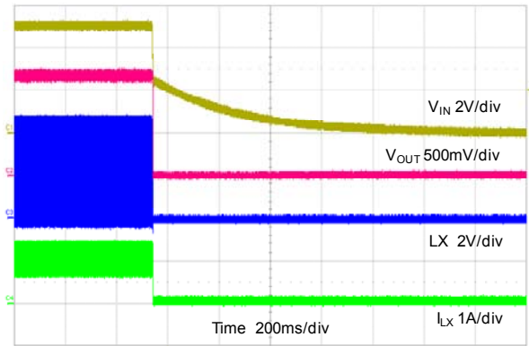
Start-down Through VIN V_{OUT}=1.2V, I_{OUT}=1A
