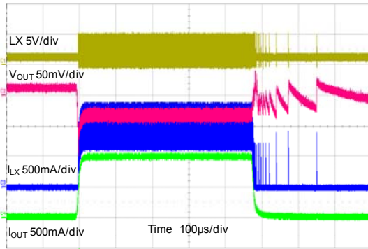
Load Transient Response V_{OUT}=1.2V, I_{OUT}=0mA \sim 1A
