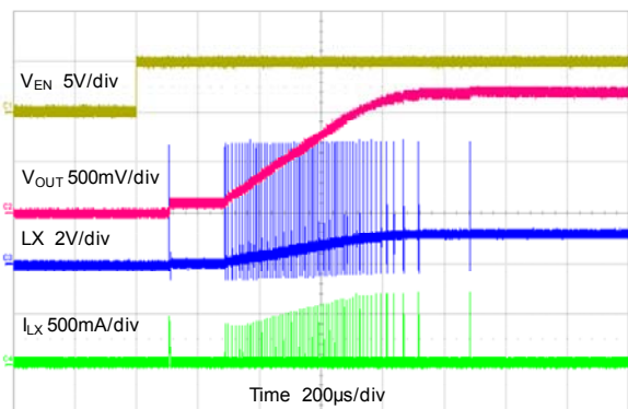
Start-up Through Enable V_{OUT}=1.2V , No Load
