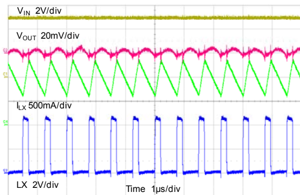
V_{OUT}=1.2V , I_{OUT}=1A
