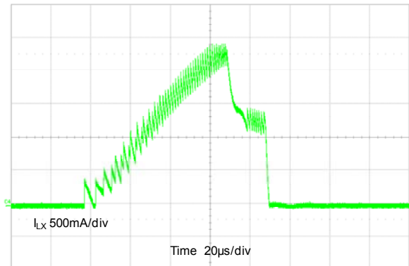
Current Limit
