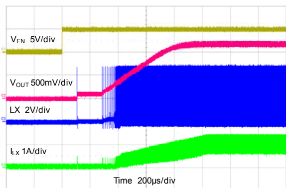
Start-up Through Enable V_{OUT}=1.2V , I_{OUT}=1A
