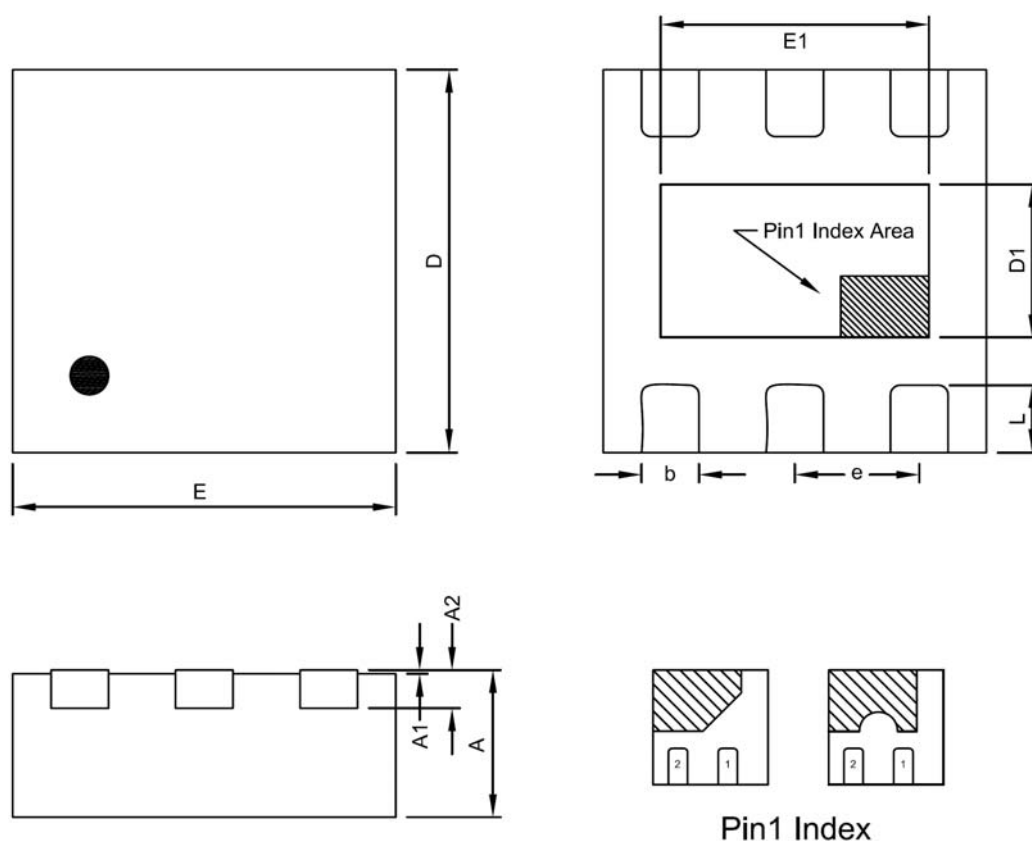
TDFN2X2-6 Package
