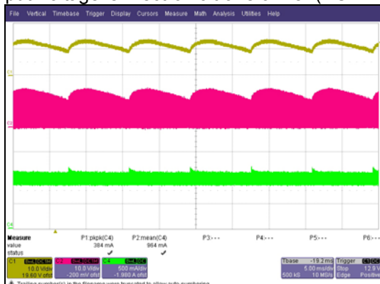
Input Voltage is Electronic transformer (AC=12V)
