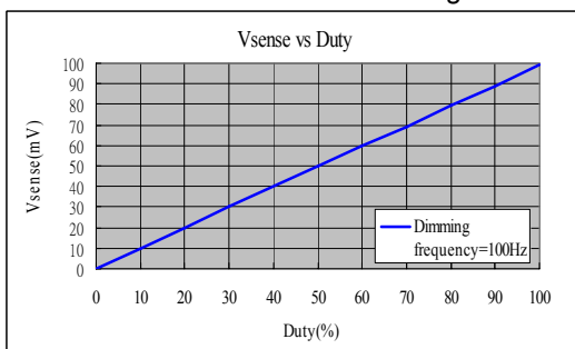
Vsense vs. PWM Dimming
