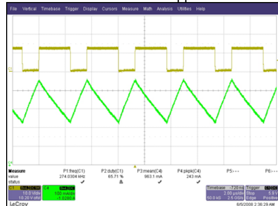
LED Current Ripple
