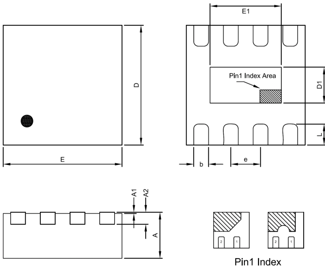
TDFN2X2-8 Package
