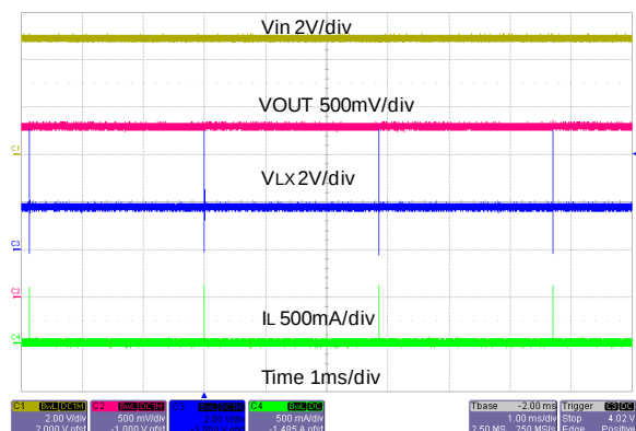
Steady State Operation ( I_o=0A )
