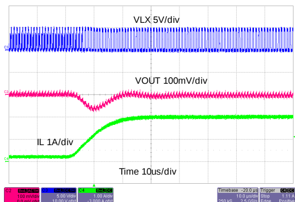
Load Transient Response (0.2A to 2A)
