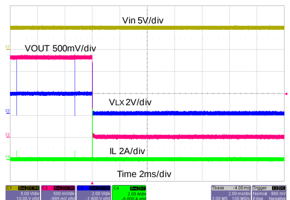
Short Circuit Waveform (Output short)
