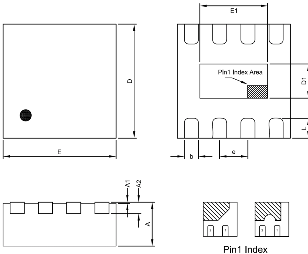
TDFN2X2-8 Package
