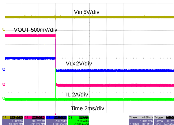
Short Circuit Waveform (Output short)
