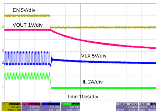
Power Off from EN ( I_o=2A )
