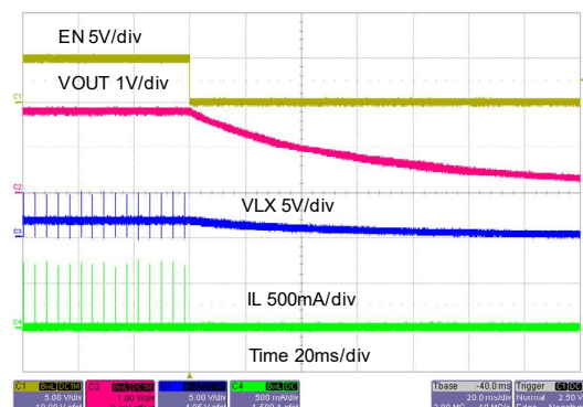
Power Off from EN ( I_o=0A )
