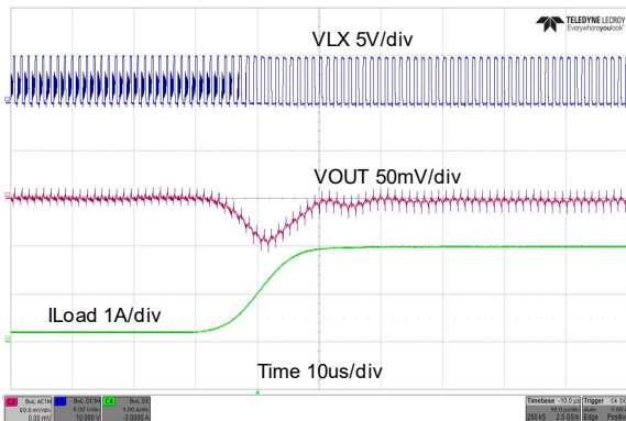
Load Transient Response (0.2A to 2A)
