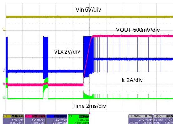
Short Circuit Waveform (Recovery)
