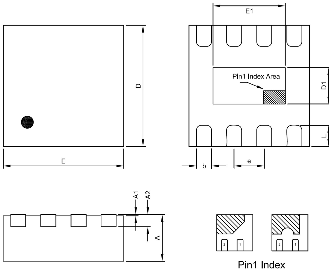
TDFN2X2-8 Package
