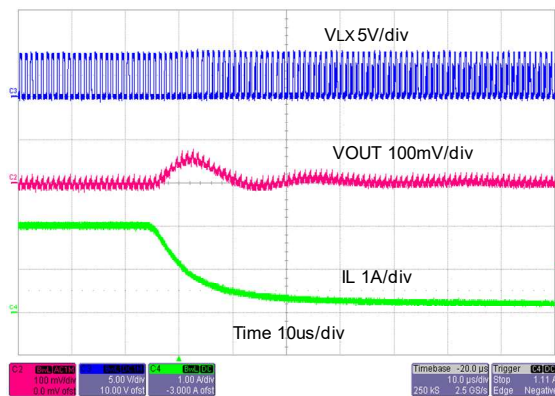
Load Transient Response (2A to 0.2A)
