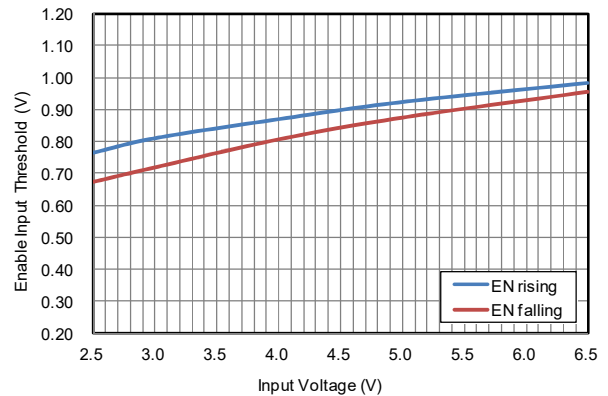
Enable input Voltage vs. Input Voltage
