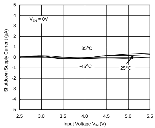
Shutdown Supply Current vs. Input Voltage
