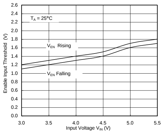
Enable Input Threshold vs. Input Voltage
