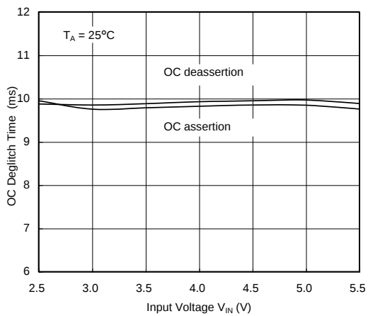
OC Deglitch Time vs. Input Voltage
