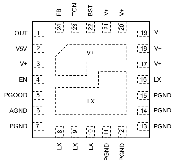
G5329B QFN3X3-24
