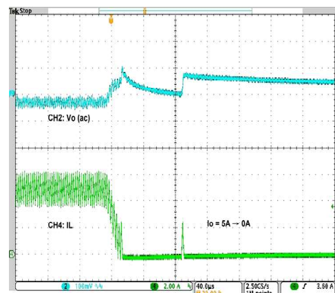
Load transient
