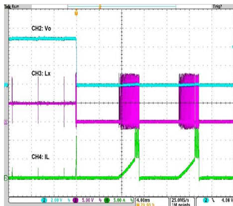
SCP
