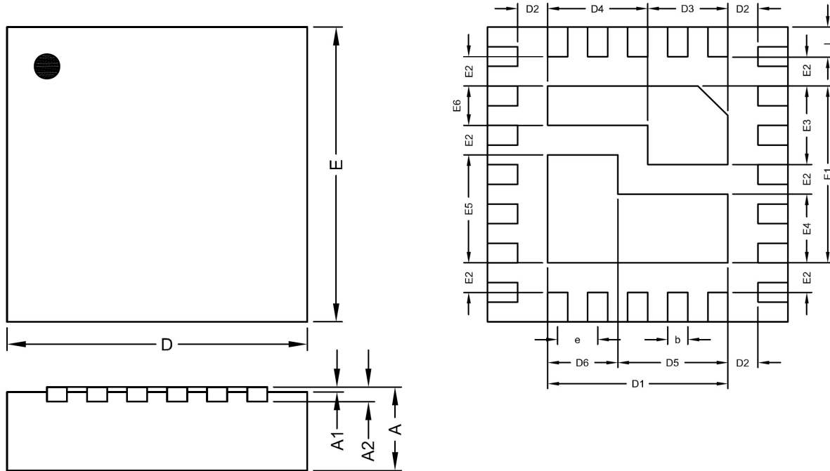
QFN3X3-24 Package
