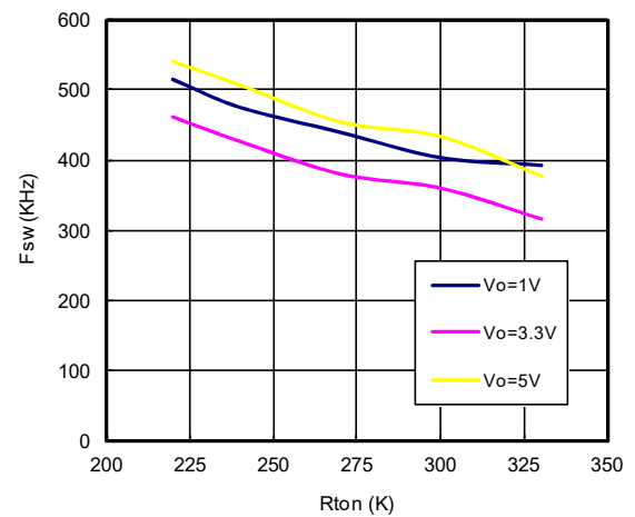
Rton vs. Fsw
