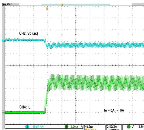
Load transient
