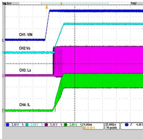
Power ON
