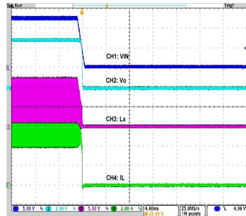
Power OFF
