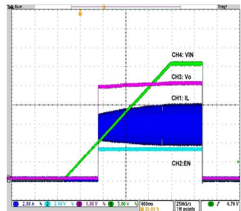
Operation with Vin Chattering
