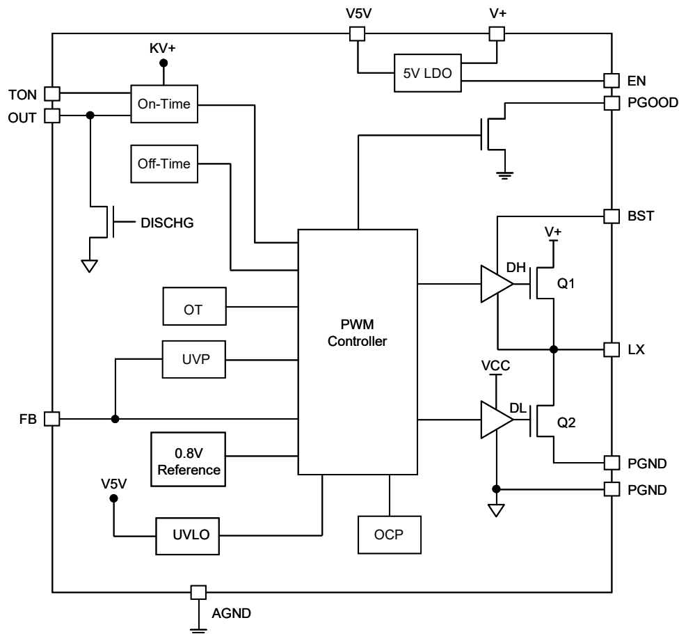
Fig. 1 Block Diagram of G5329B
