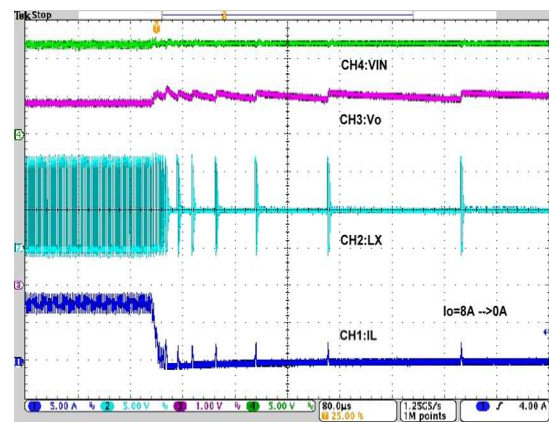
Load transient
