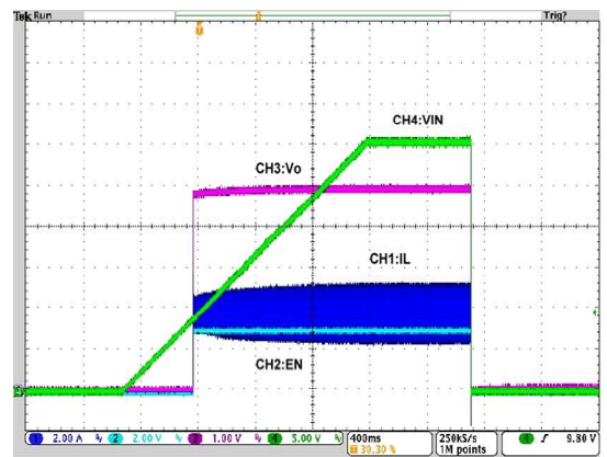
Operation with Vin Chattering
