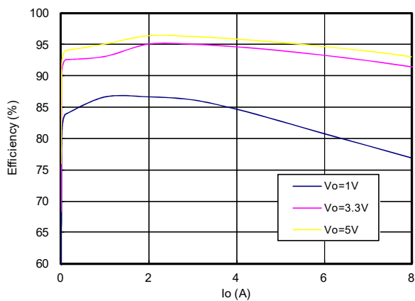
Efficiency
