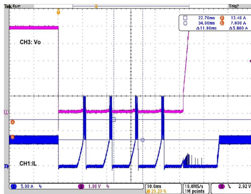
SCP
