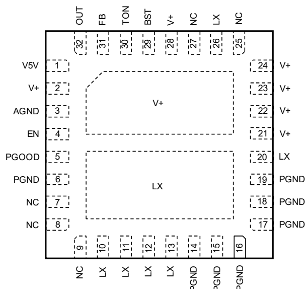
G5329 QFN4X4-32
