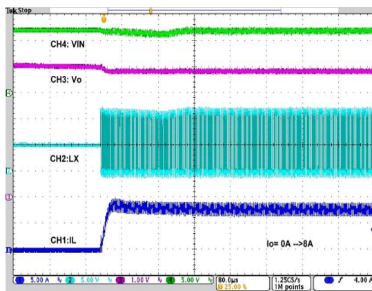
Load transient
