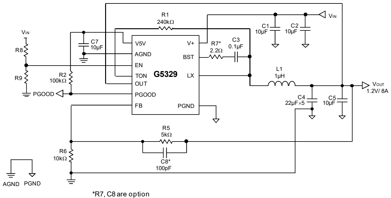
Fig. 2-A Standard Application Circuit
