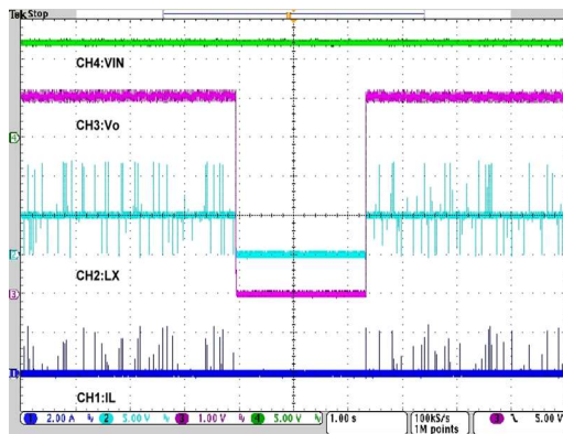
OTP
