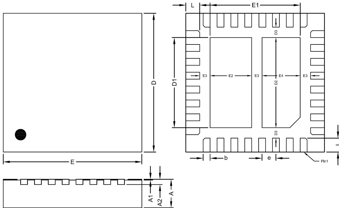
QFN4X4-32 Package
