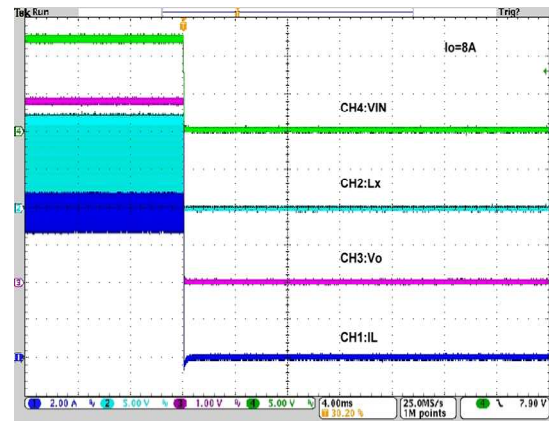
Power OFF
