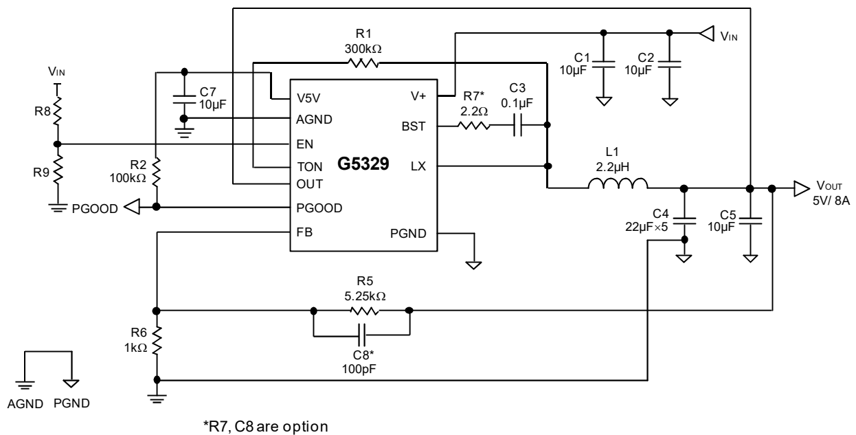
Fig. 2-B Standard Application Circuit
