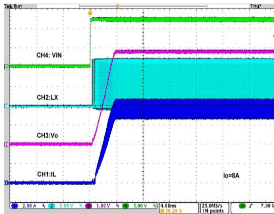
Power ON
