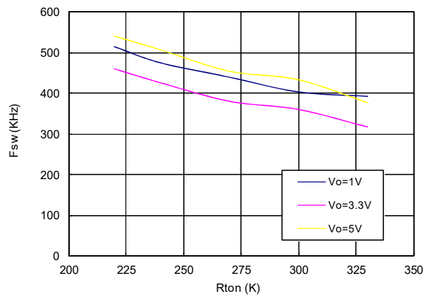
Rton vs. Fsw
