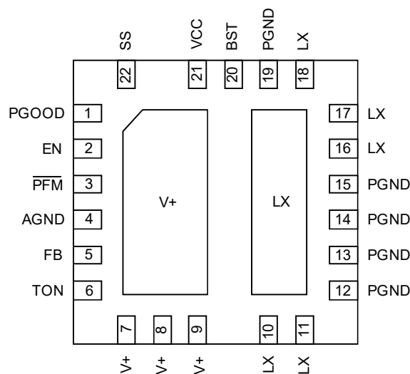
G5335D QFN4X4-22
