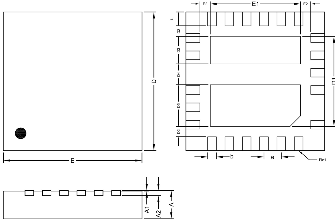
QFN4X4-22 Package
