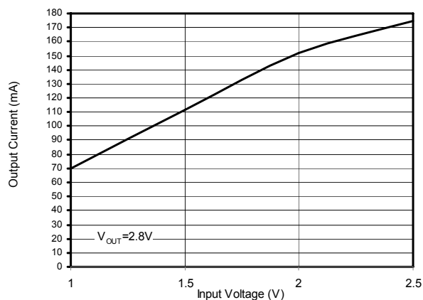
Maximun Output Current vs. Input Voltage
