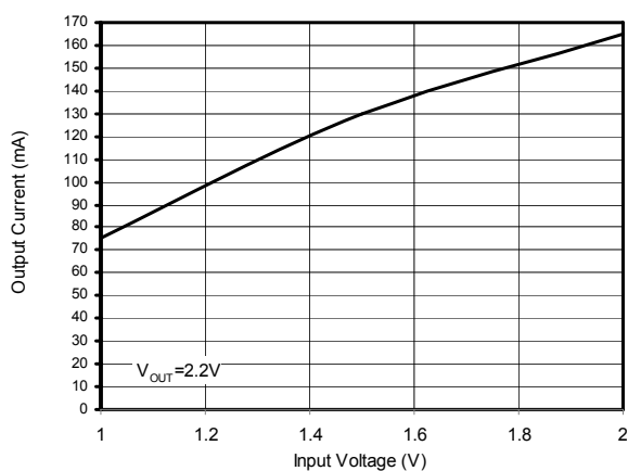
Maximun Output Current vs. Input Voltage
