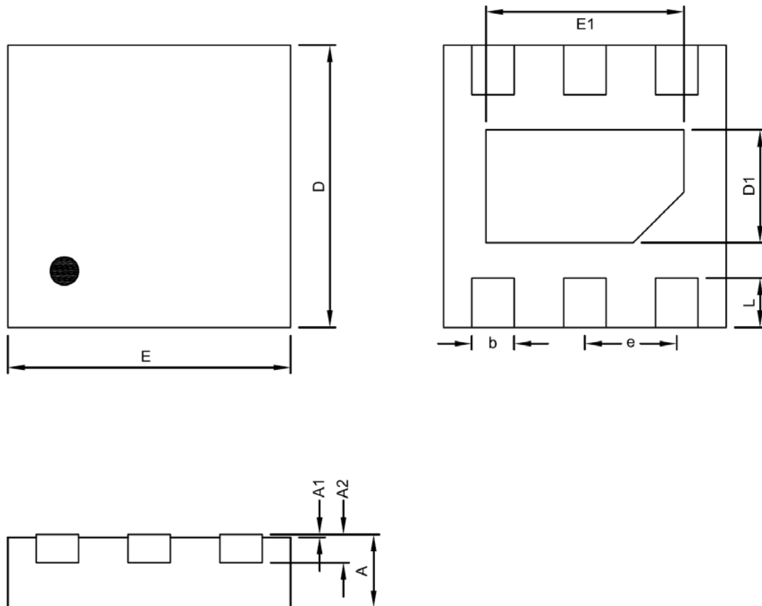
WDFN2X2-6 Package
