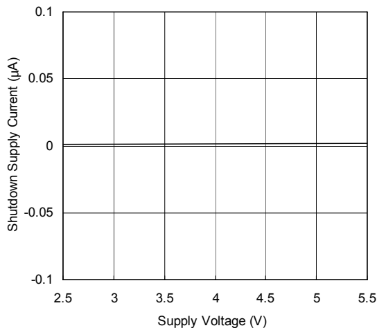
Shutdown Supply Current vs Supply Voltage
