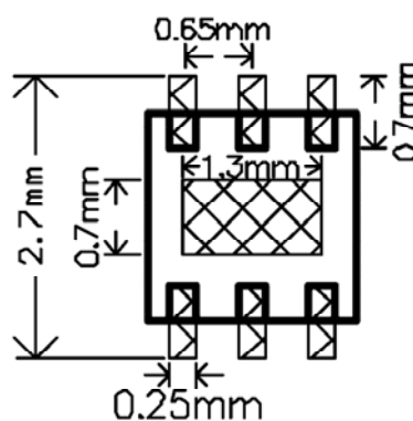
WDFN2X2-6
