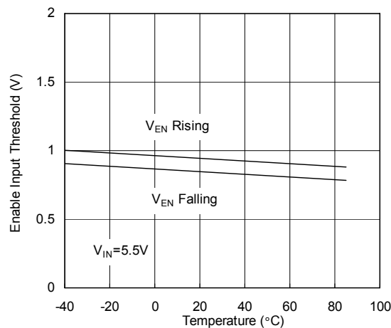
Enable Input Threshold vs Temperature
