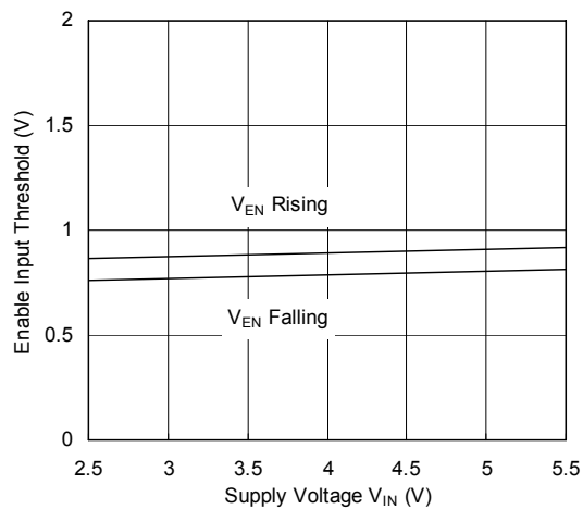
Enable Input Threshold vs Supply Voltage
