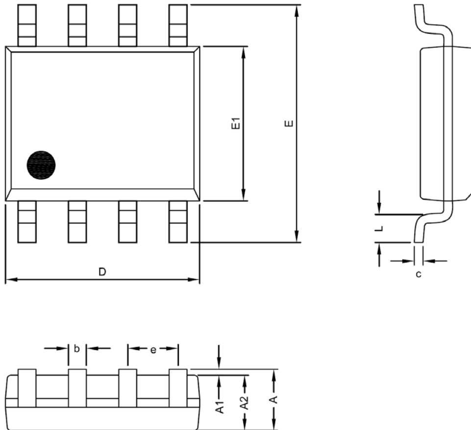
SOP-8 Package
