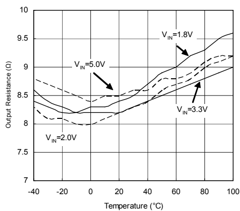
Output Resistance vs. Temperature
