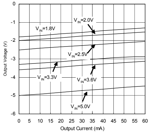
Output Voltage vs. Current
