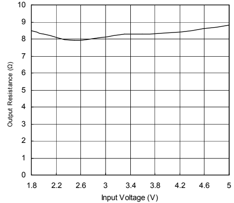
Output Resistance vs. Input Voltage
