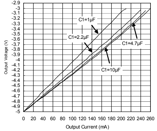
Output Voltage vs Output Current at V_{IN}=+5V
