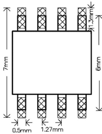
SOP-8
