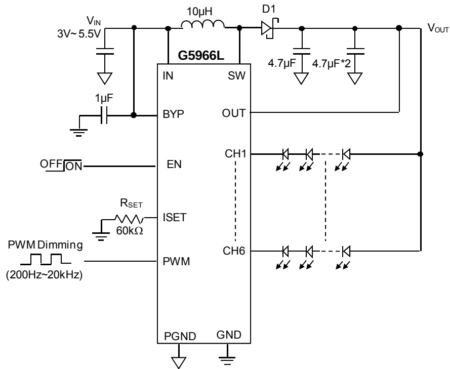
Fig. 3 Ultra Low VIN Application with BYP connected to VIN
