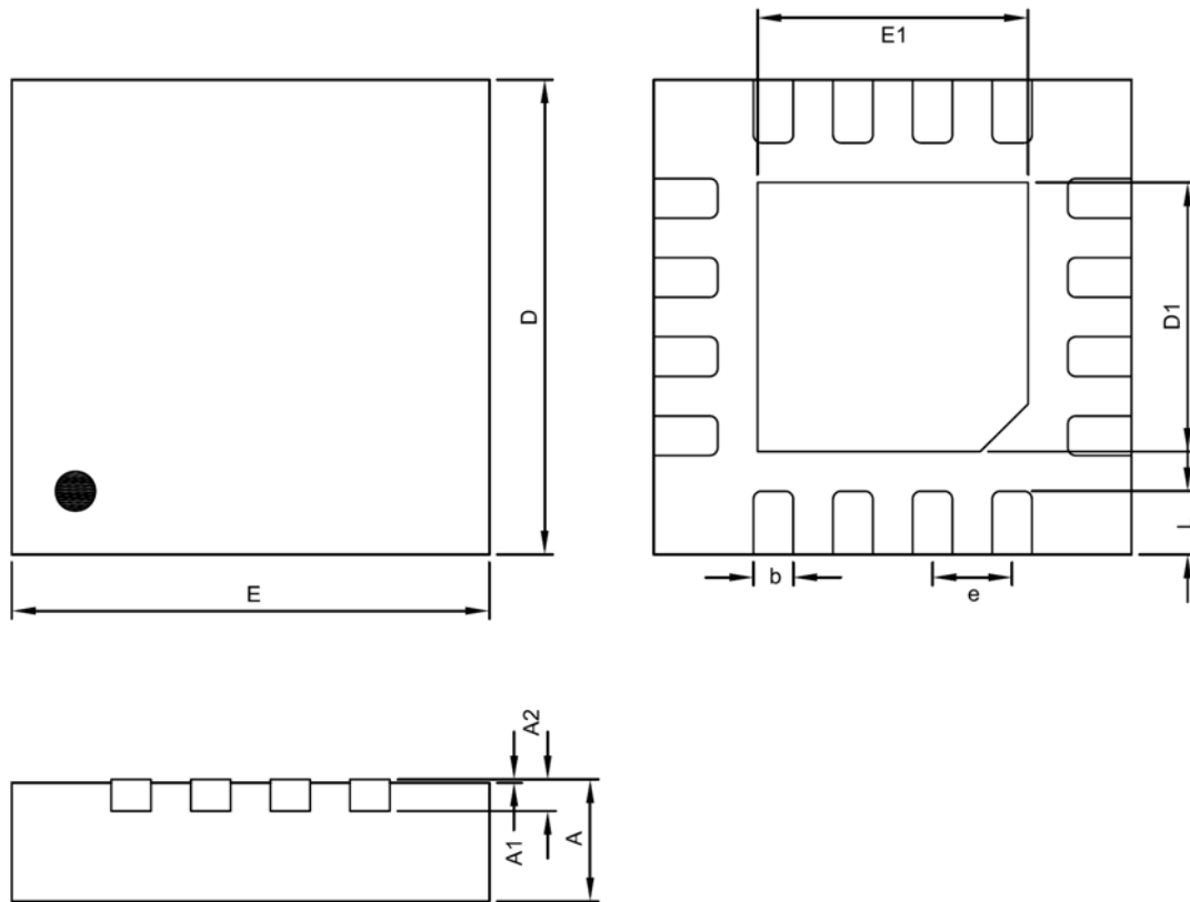
TQFN3X3-16 Package
