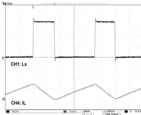
Lx – rise / fall time
