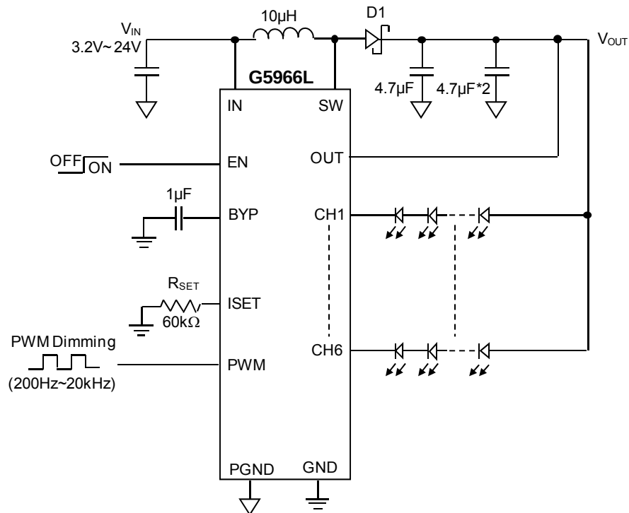
Fig.1 Typical Application
