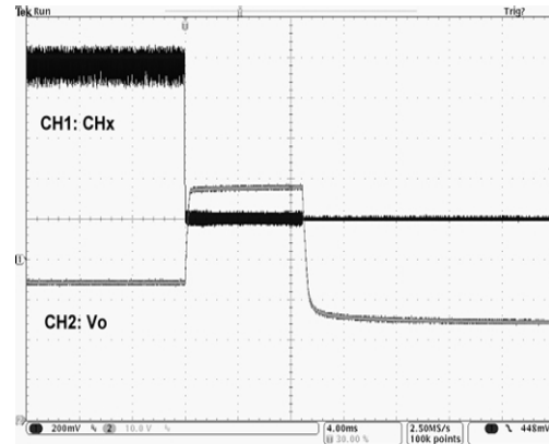
SCP (Short Circuit Protection)
