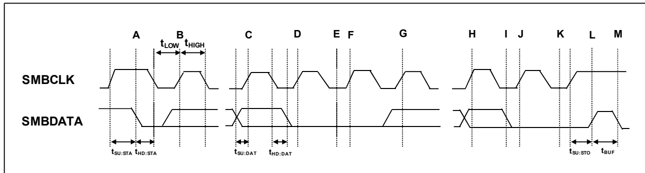
Figure 1. SMBus Write Timing Diagram
