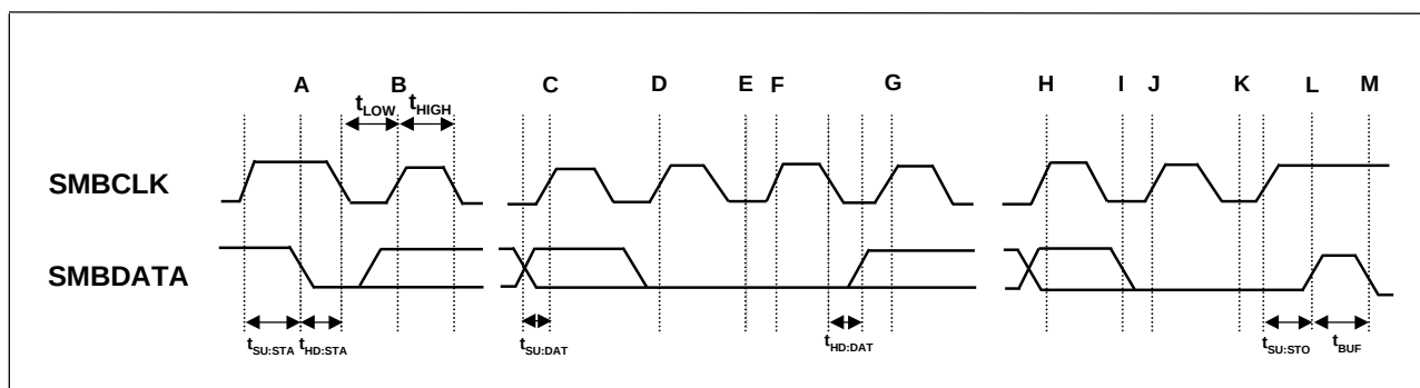
Figure 9. SMBus Write Timing Diagram
