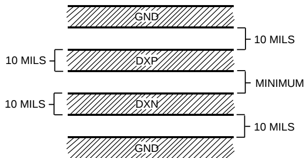
Figure 3. Recommended DXP/DXN PC Traces
