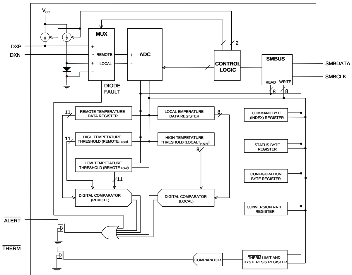
Figure 1. Functional Diagram
