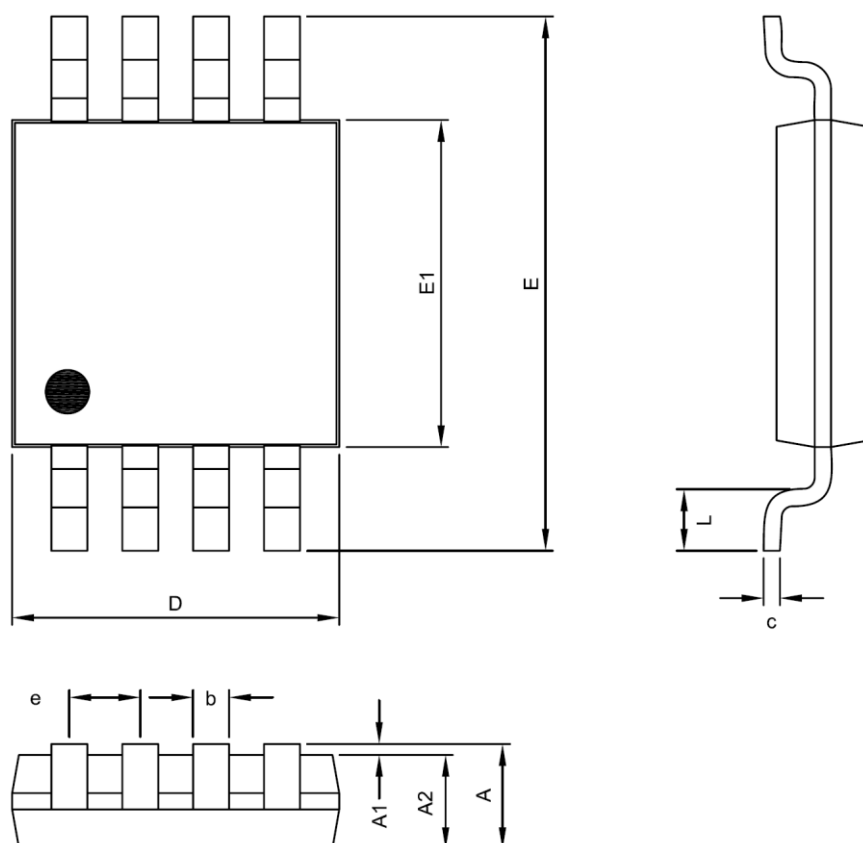
MSOP-8 Package
