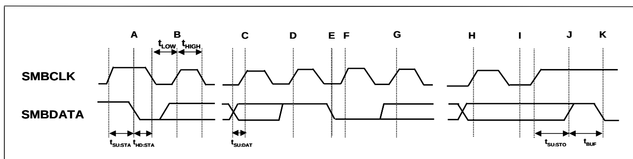
Figure 10. SMBus Read Timing Diagram
