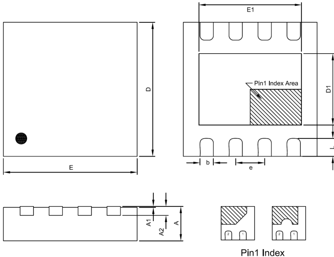
TDFN3X3-8 Package
