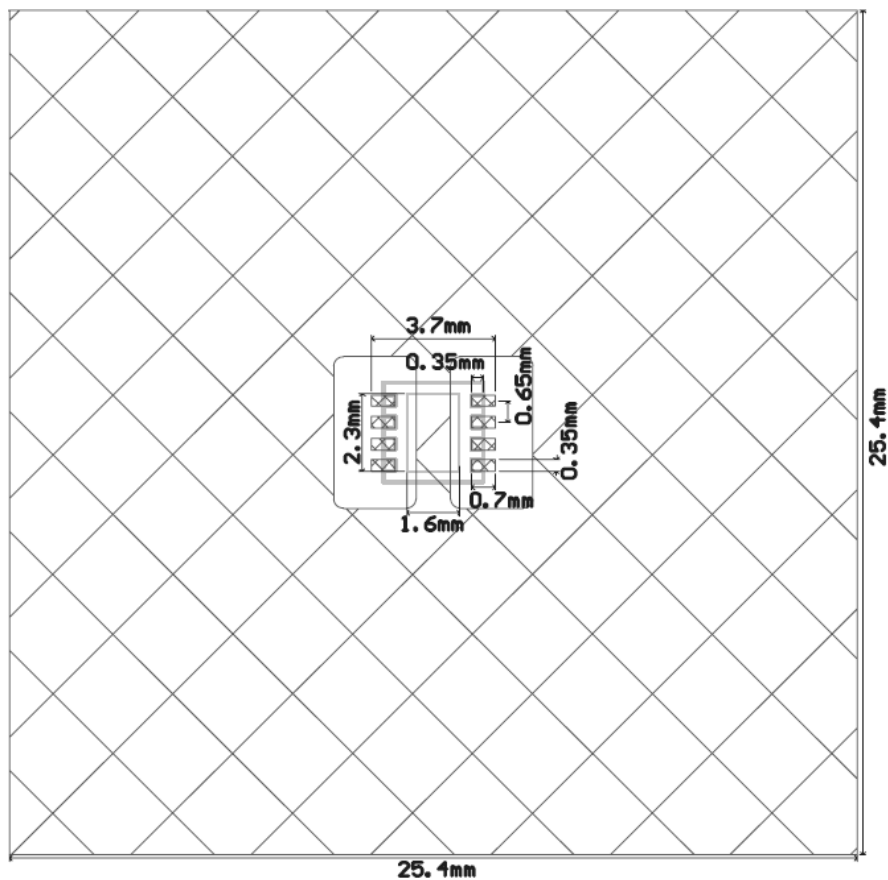
TDFN3X3-8
