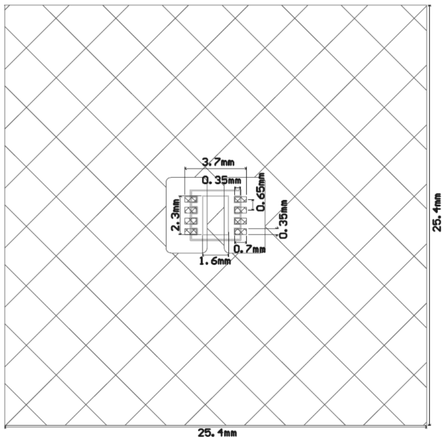
TDFN3X3-8
