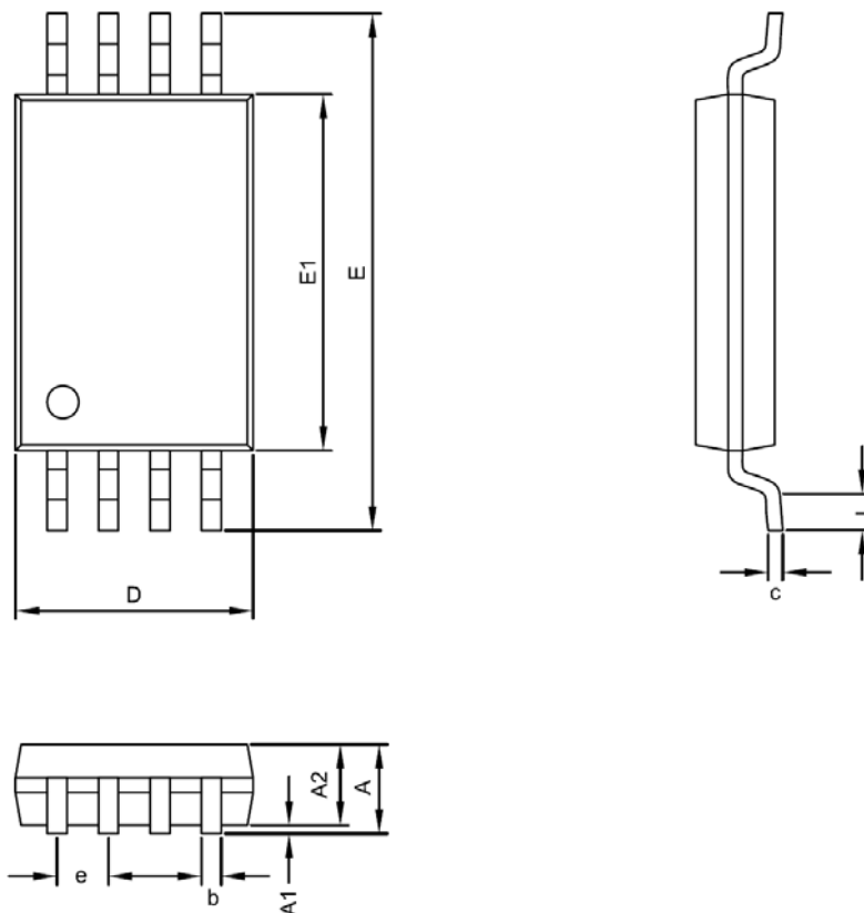
TSSOP-8 Package
