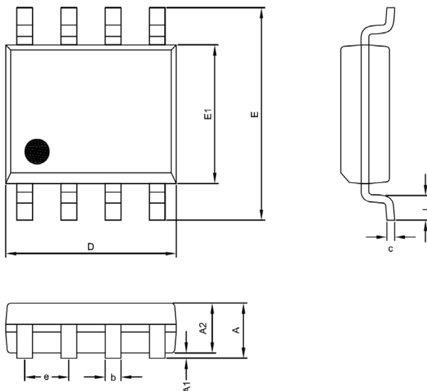
SOP-8 Package
