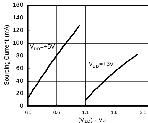
Sourcing Current vs. (V_{DD}) - V_O
