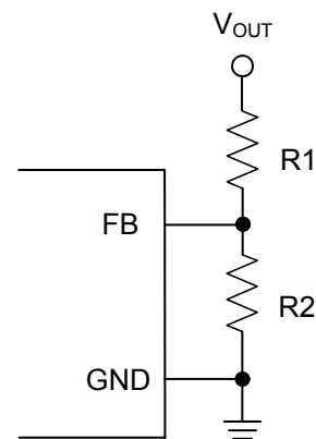
Figure 1. Setting V OUT with a Voltage Divider
