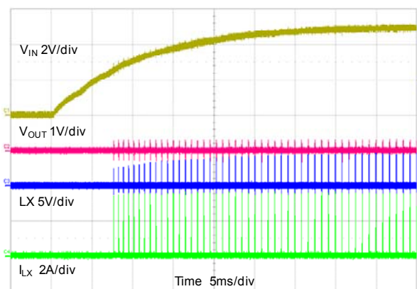
Short Circuit waveform V_{OUT}=1.8V
