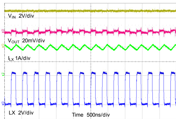
Steady State Operation V_{OUT}=1.8V , I_{OUT}=2A
