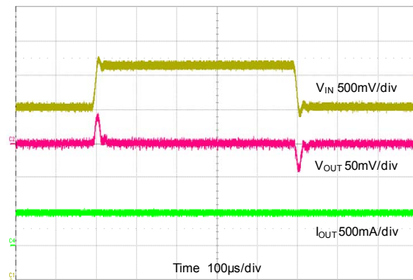
Line Transient Response V_{IN}=3.6V\sim4.2V, V_{OUT}=1.8V, I_{OUT}=500mA
