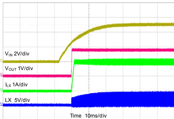
Start-up Through VIN V_{OUT}=1.8V, I_{OUT}=2A
