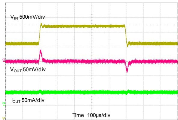
Line Transient Response V_{IN}=3.6V\sim4.2V, V_{OUT}=1.8V, I_{OUT}=50mA
