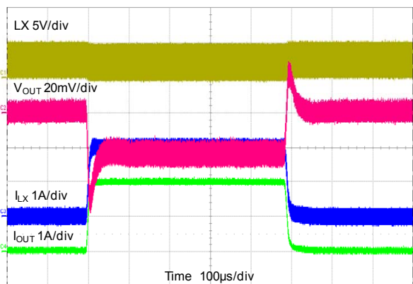
Load Transient Response V_{OUT}=1.8V, I_{OUT}=0mA\sim2A (PWM mode)
