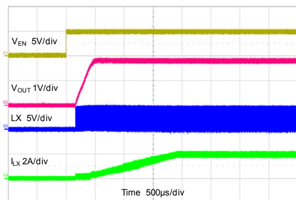
Start-up Through Enable V_{OUT}=1.8V , I_{OUT}=2A
