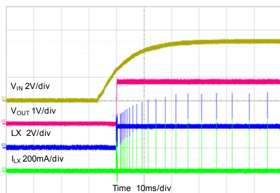
Start-up Through VIN V_{OUT}=1.8V , No Load
