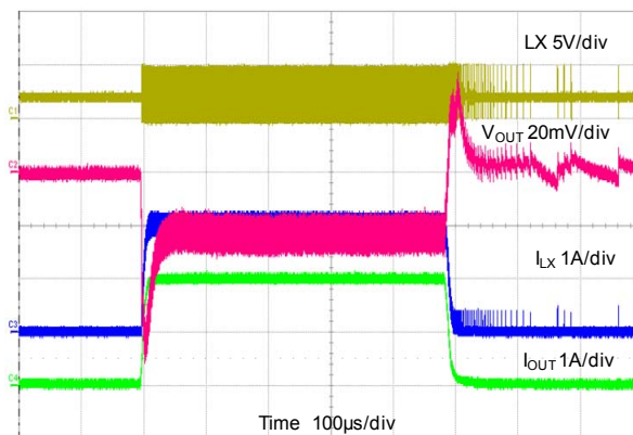
Load Transient Response V_{OUT}=1.8V, I_{OUT}=0mA\sim2A (PSM mode)
