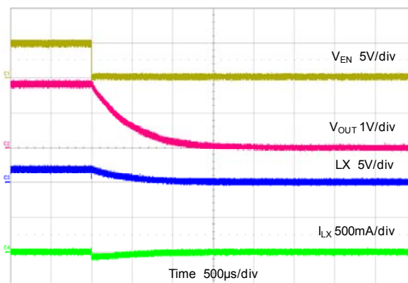
Start-down Through Enable V_{OUT}=1.8V , No Load
