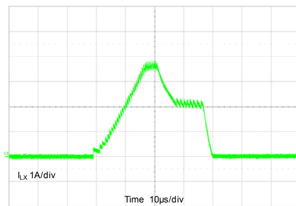
Current Limit V_{OUT}=1.8V
