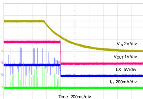
Start-down Through VIN V_{OUT}=1.8V , No Load
