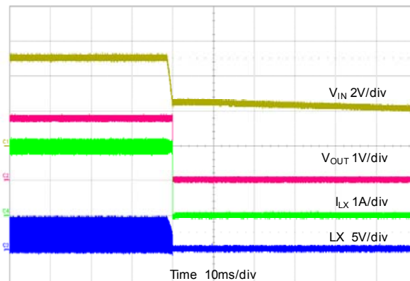
Start-down Through VIN V_{OUT}=1.8V, I_{OUT}=2A
