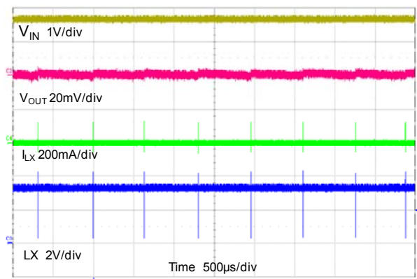
Steady State Operation V_{IN}=3.7V , V_{OUT}=3.3V , No Load
