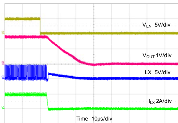
Start-down Through Enable V_{OUT}=1.8V , I_{OUT}=2A
