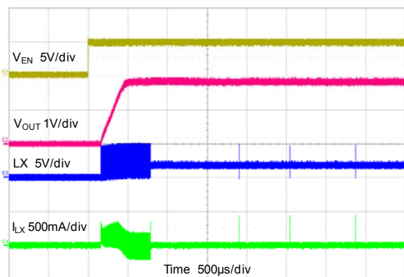
Start-up Through Enable V_{OUT}=1.8V , No Load
