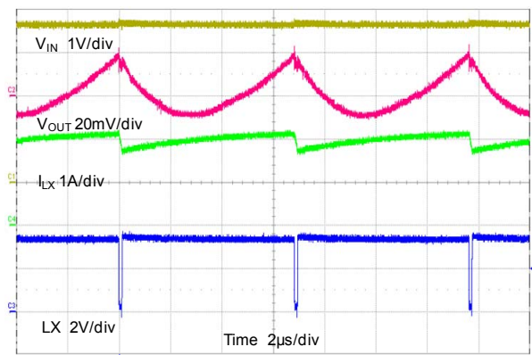
Steady State Operation V_{IN}=3.7V , V_{OUT}=3.3V , I_{OUT}=2A
