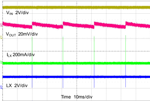
Steady State Operation V_{OUT}=1.8V , No Load
