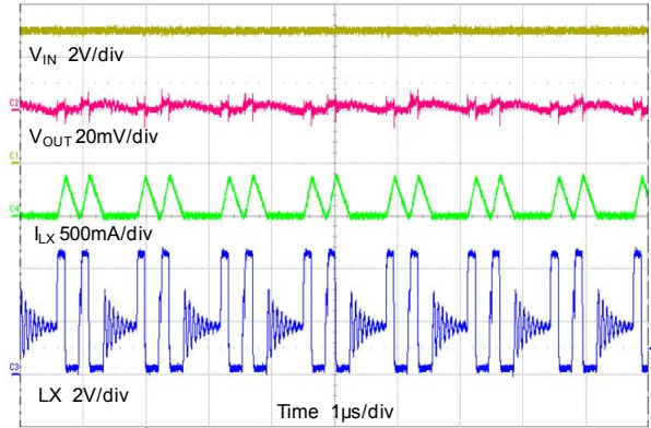
Steady State Operation V_{OUT}=1.8V , I_{OUT}=100mA
