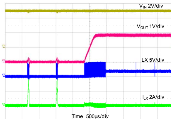
Short Circuit Recovery V_{OUT}=1.8V
