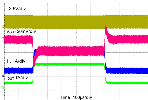
Load Transient Response V_{OUT}=1.8V, I_{OUT}=500mA\sim2A
