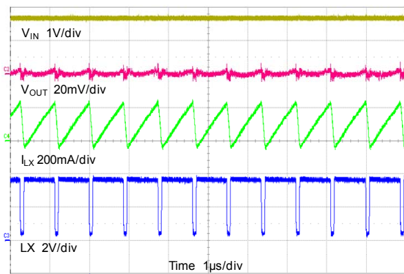
Steady State Operation V_{IN}=3.7V , V_{OUT}=3.3V , I_{OUT}=100mA
