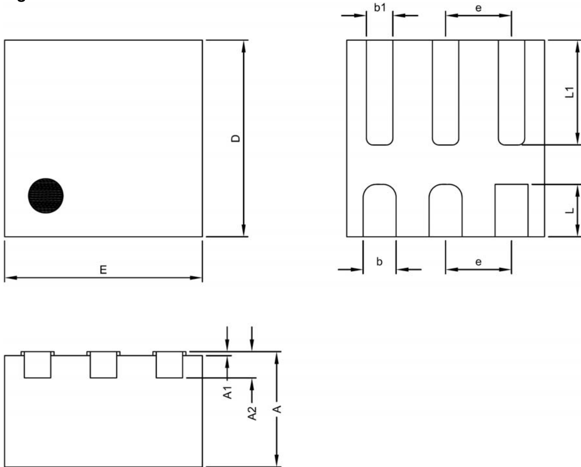
ADFN1.5X1.5-6 Package
