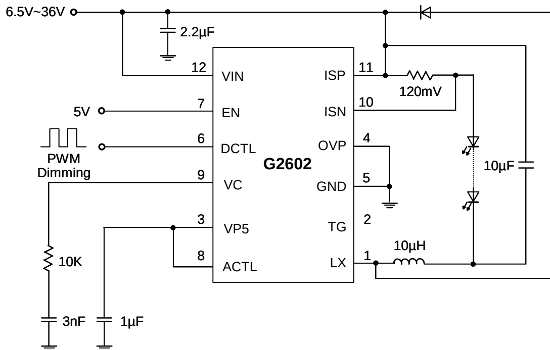
Fig. 3 PWM Dimming BUCK Configuration
