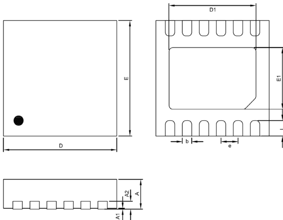
TDFN3X3-12 Package
