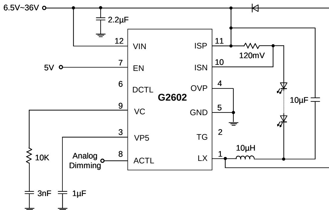
Fig. 2 Analog Dimming BUCK Configuration
