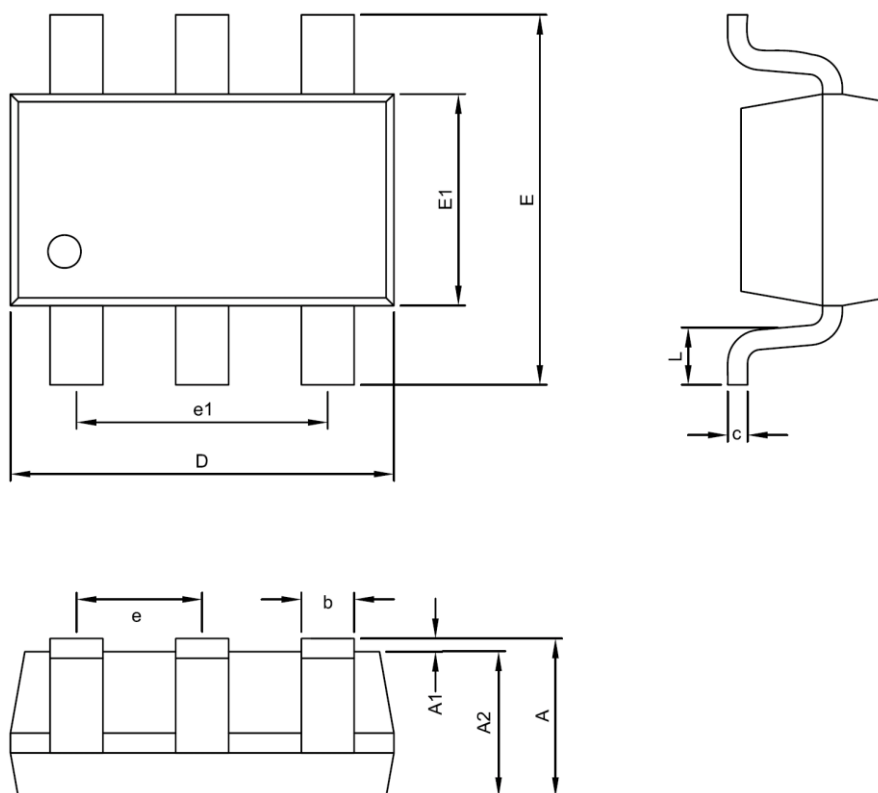
SOT-23-6 Package
