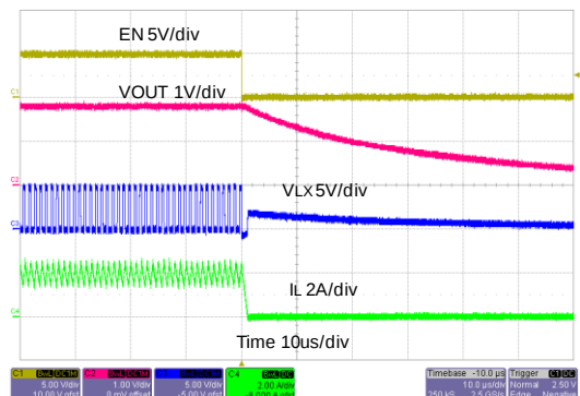
Power Off from EN ( I_o=2A )
