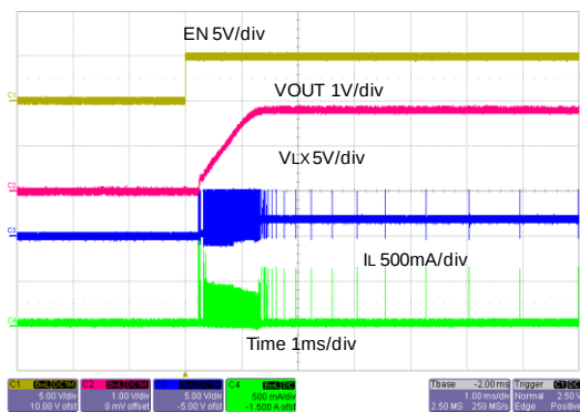
Power On from EN ( I_o=0A )
