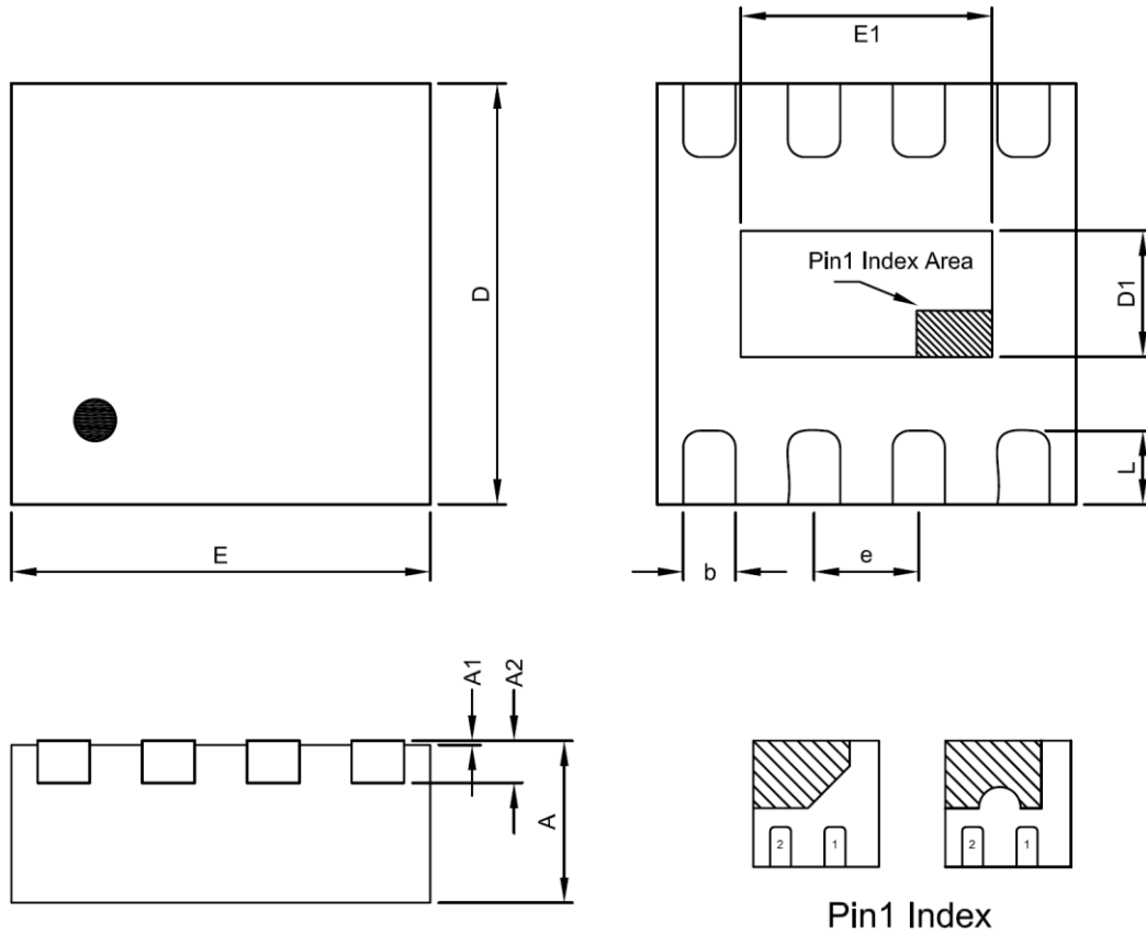
TDFN2X2-8 Package
