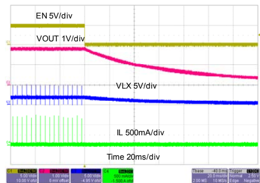
Power Off from EN ( I_o=0A )
