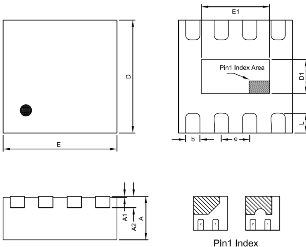
TDFN2X2-8 Package
