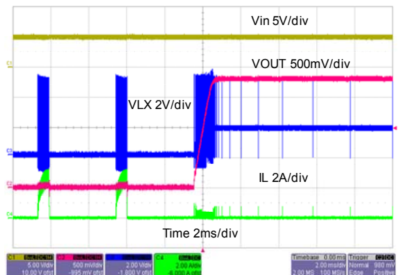
Short Circuit Waveform (Recovery)
