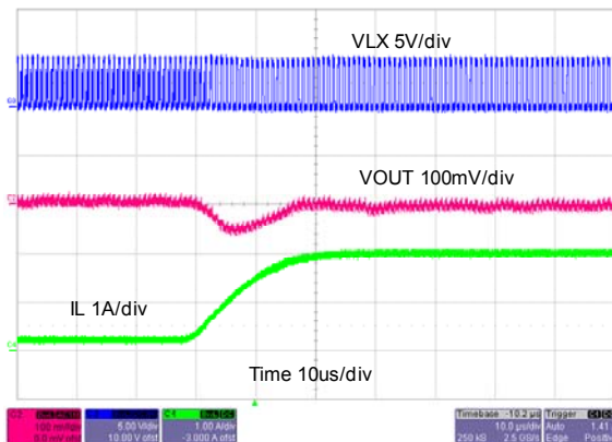
Load Transient Response (0.2A to 2A)
