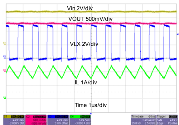
Steady State Operation ( I_o=2A )
