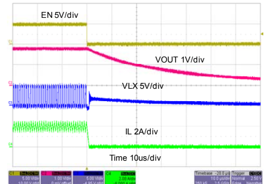
Power Off from EN ( I_o=2A )
