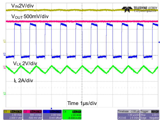
Steady State Operation V_{IN}=5V , V_{OUT}=1.8V , I_O=4A
