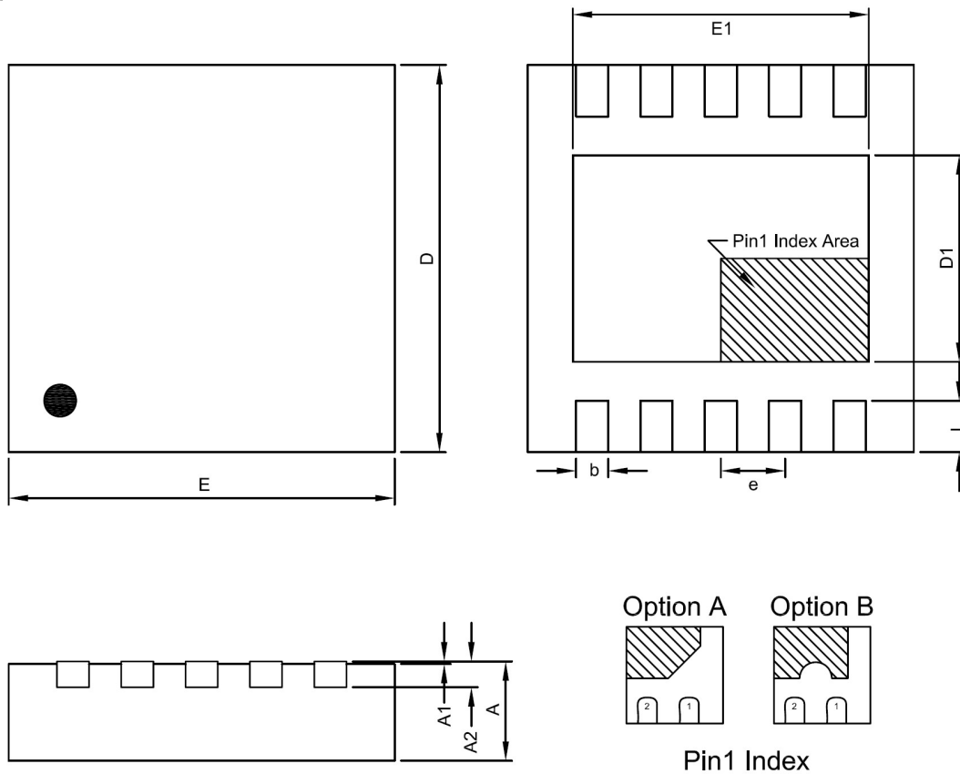
TDFN3X3-10 Package
