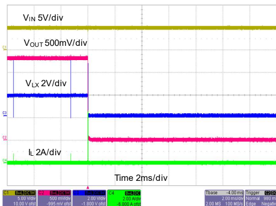
Short Circuit Waveform (Output short)
