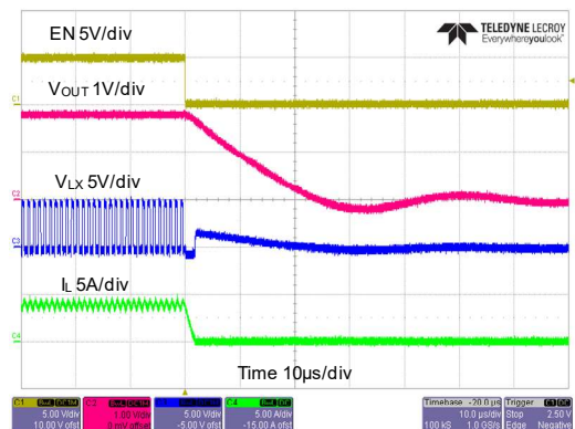
Power OFF from EN ( I_o=4A ) V_{IN}=5V , V_{OUT}=1.8V , I_o=2A , EN off
