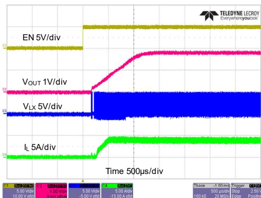
Power ON from EN ( I_o=4A ) V_{IN}=5V , V_{OUT}=1.8V , I_o=2A , EN on
