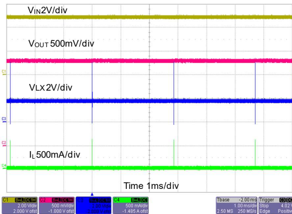
Steady State Operation ( I_O=0A )
