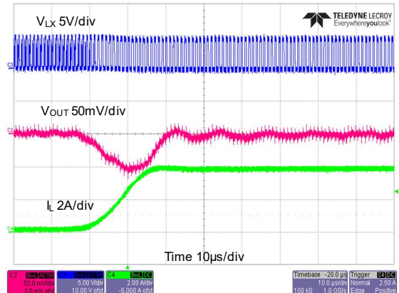
Load Transient Response V_{IN}=5V , V_{OUT}=1.8V , I_O=4A \sim 0.2A .
