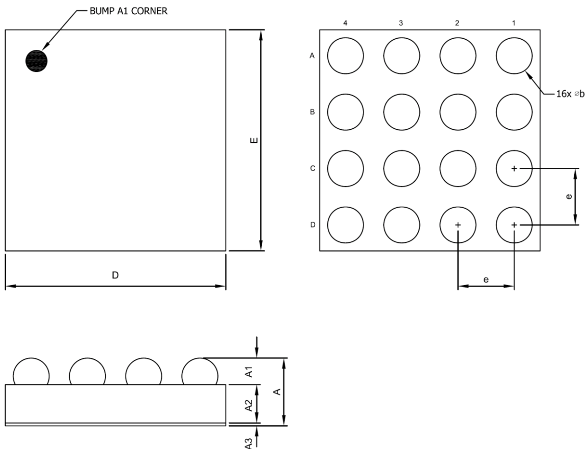
WLCSP4X4-16 Package
