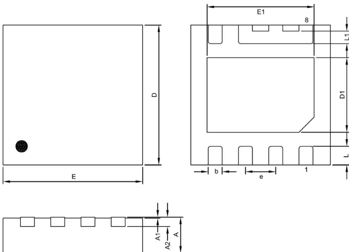
TDFN3X3-8 Package
