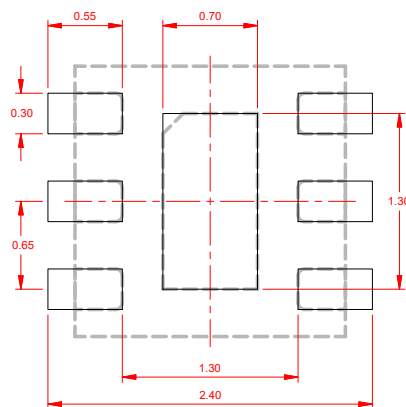
TDFN2X2-6
