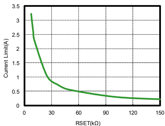
Current Limit vs. RSET
