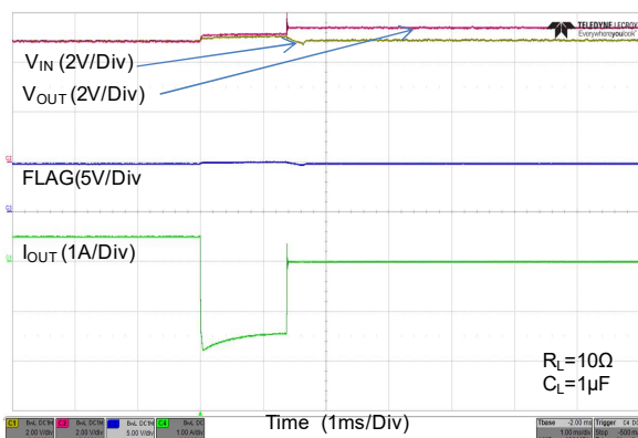
Reverse Current Protection
