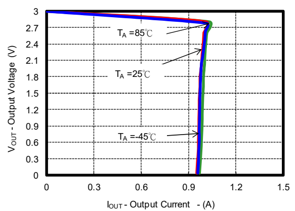
Over Current Protection Characteristics
