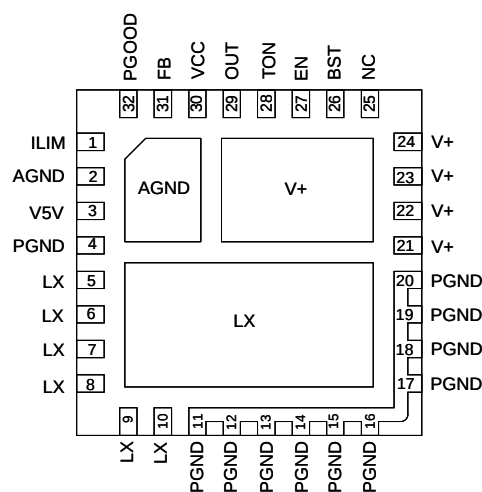
G5309 QFN5X5-32
