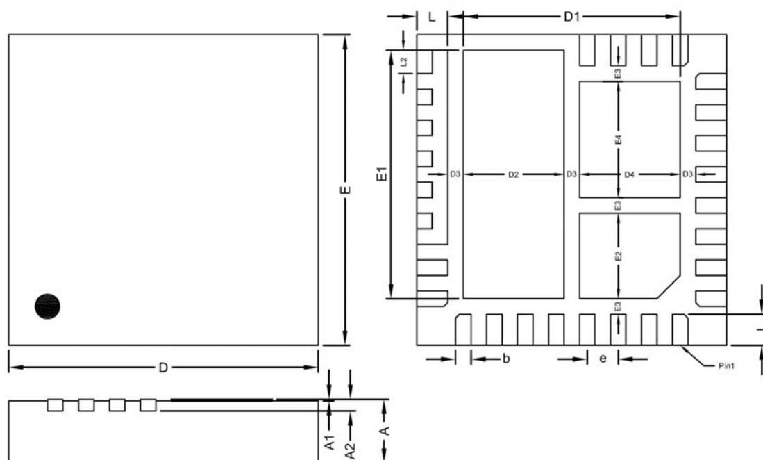
QFN4X4-28 Package
