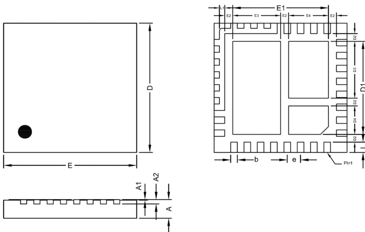
QFN5X5-32 Package
