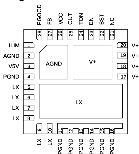
G5309 QFN4X4-28
