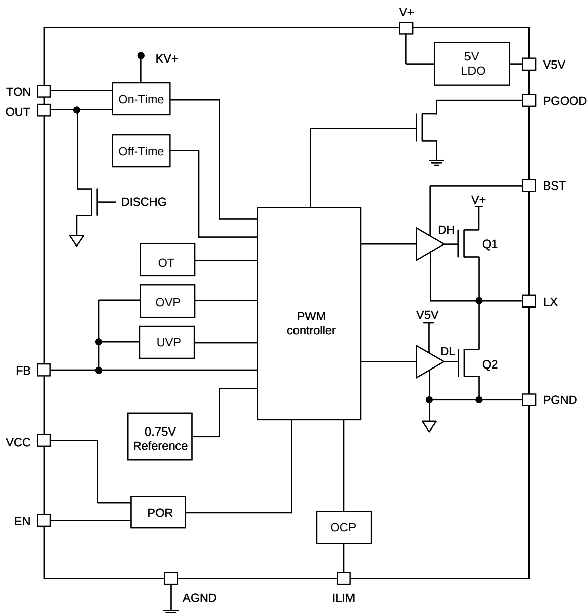
Fig. 2 Block Diagram of G5309
