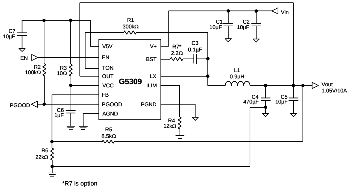
Fig. 1-A Standard Application Circuit
