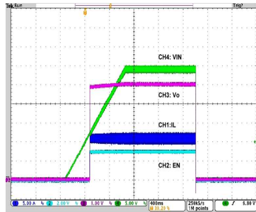
Operation with Vin Chattering
