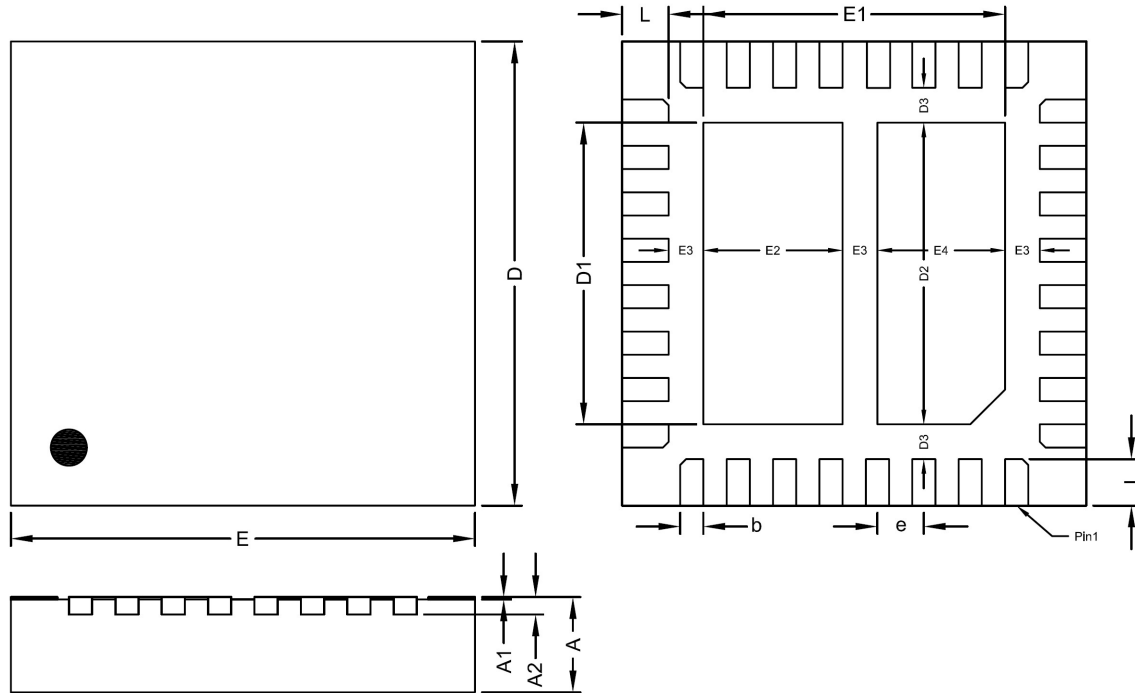
QFN4X4-32 Package
