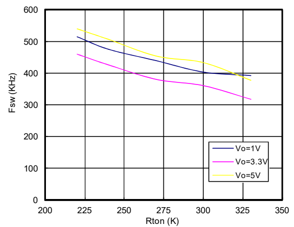
Rton vs. Fsw
