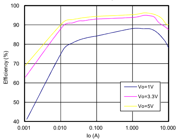
Efficiency
