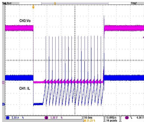
SCP
