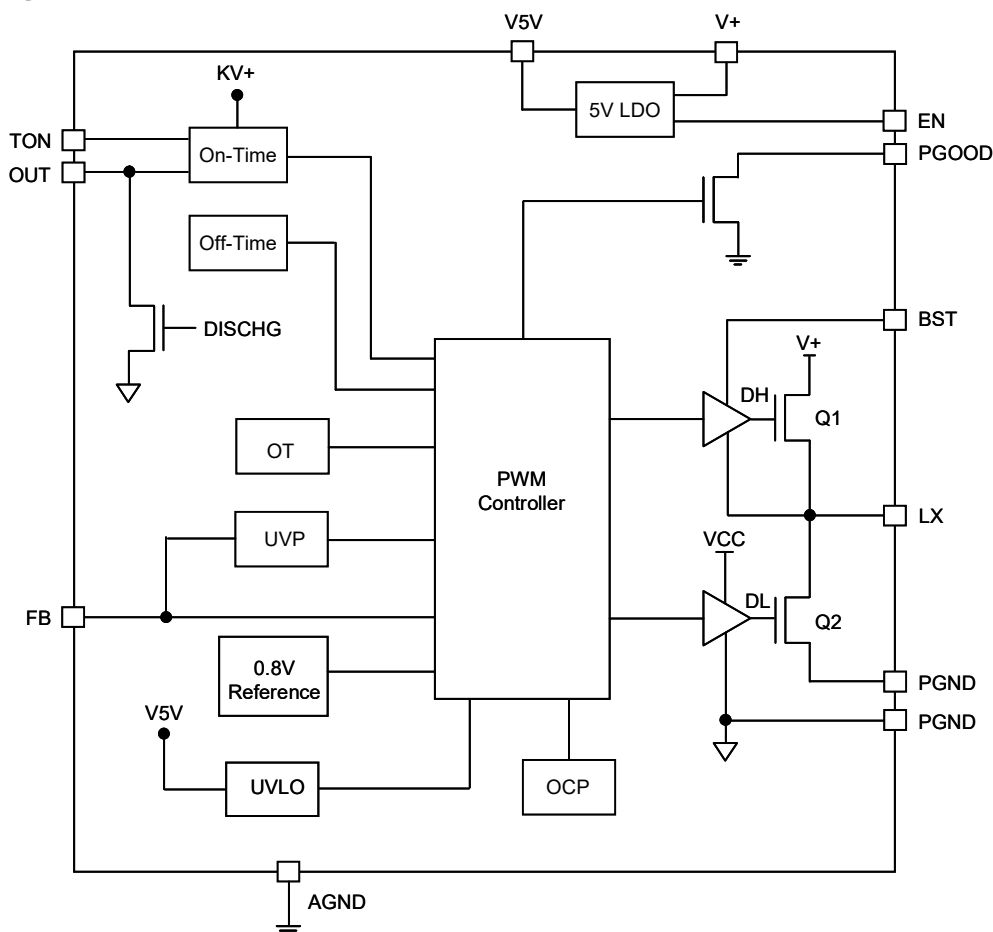
Fig. 1 Block Diagram of G5329A
