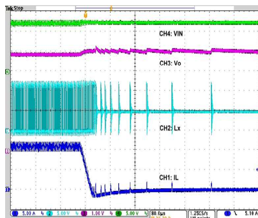
Load transient
