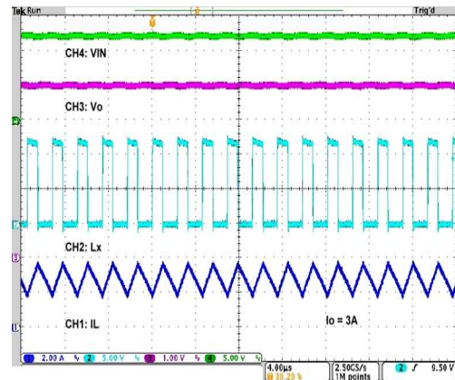
Stability
