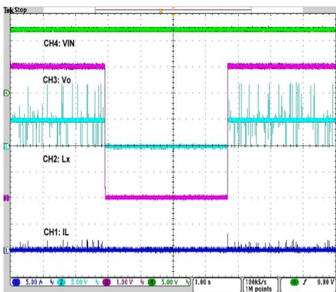
OTP
