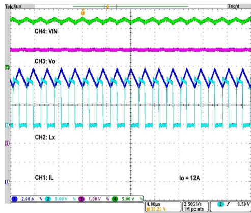
Stability
