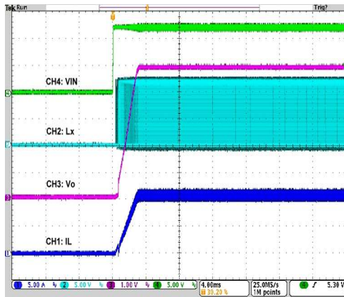
Power ON
