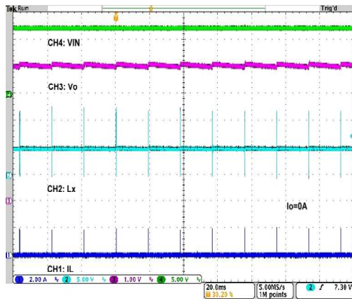
Stability
