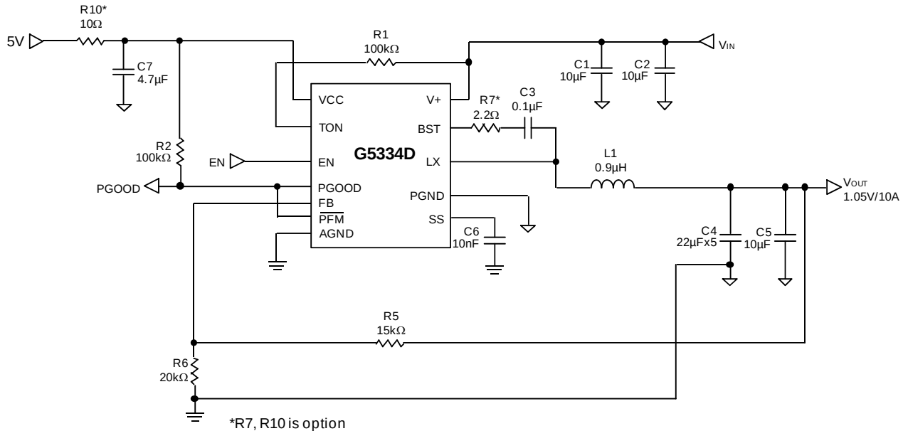
Fig. 1-C Application Circuit with Forced PWM Mode
