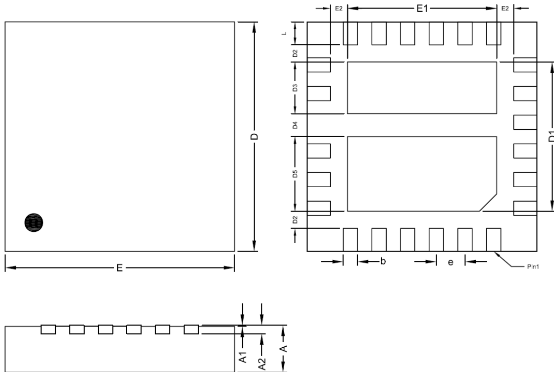
QFN4X4-23 Package
