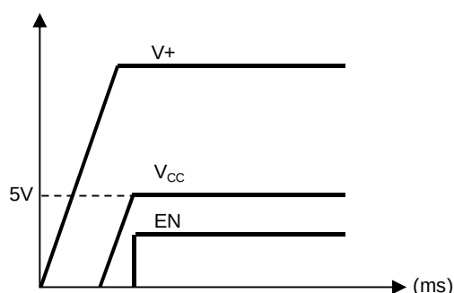
Fig. 4 Power-on Sequence
