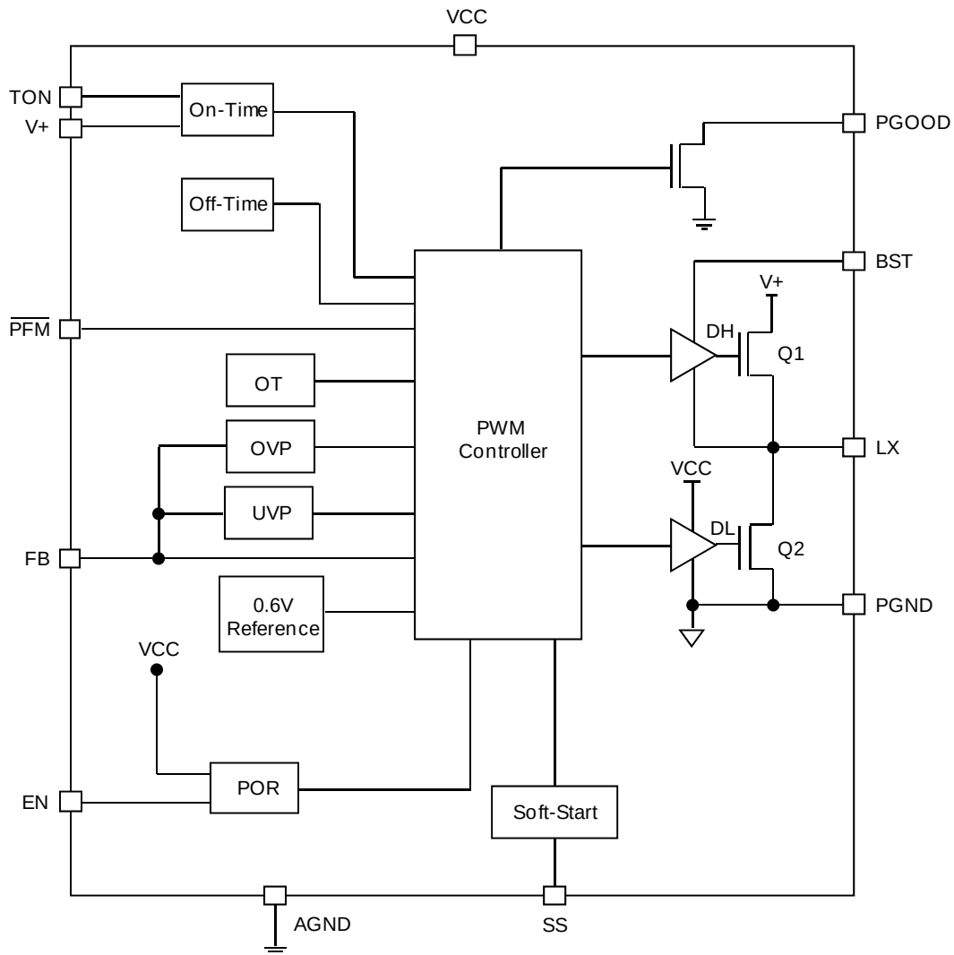
Fig. 2 Block Diagram of G5334D
