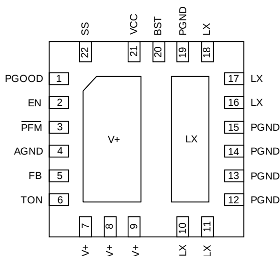
G5335C QFN4X4-22
