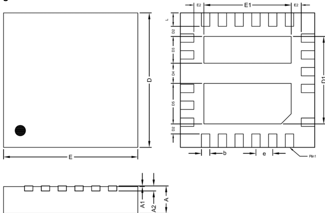
QFN4X4-22 Package
