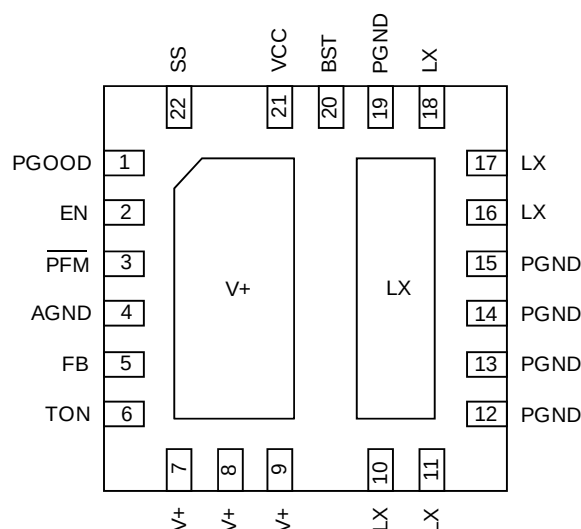
G5335F QFN4X4-22
