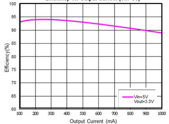
Efficiency vs. Output Current ( V_{IN}=5V )
