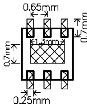
TDFN2X2-6
