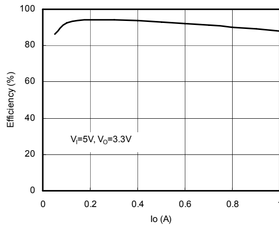
Efficiency vs. I O
