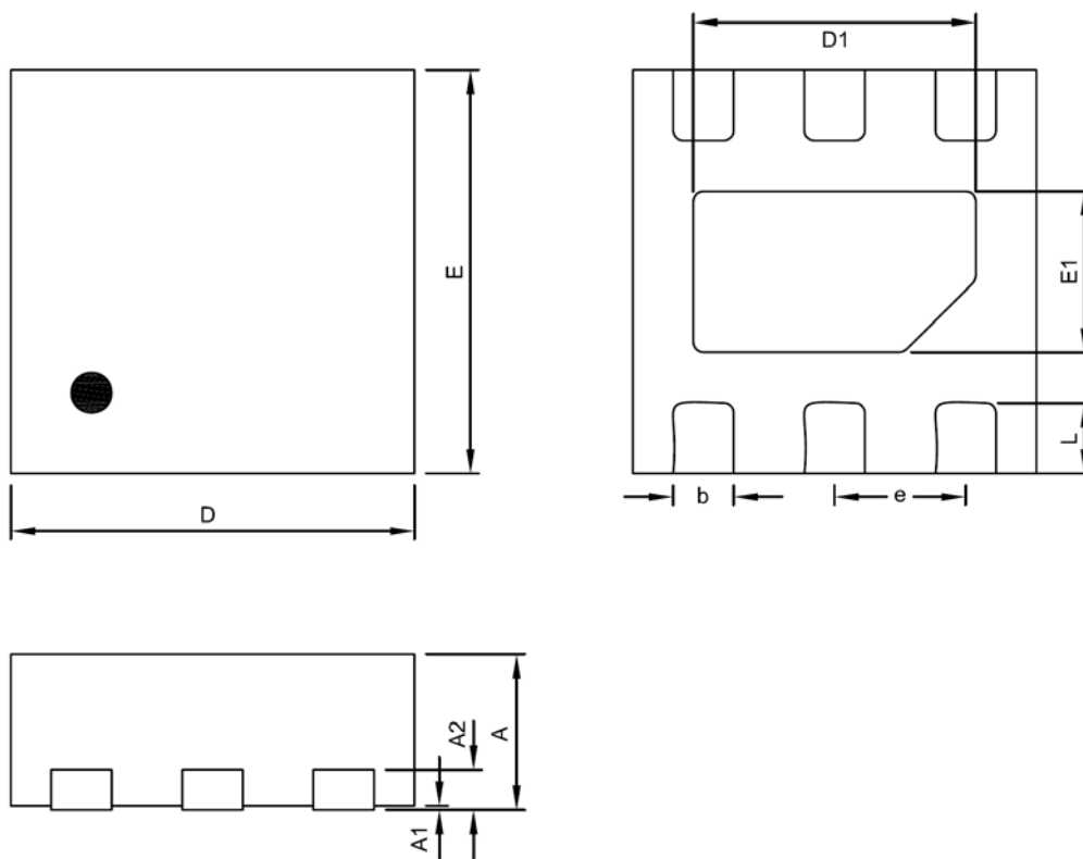
TDFN2X2-6 Package
