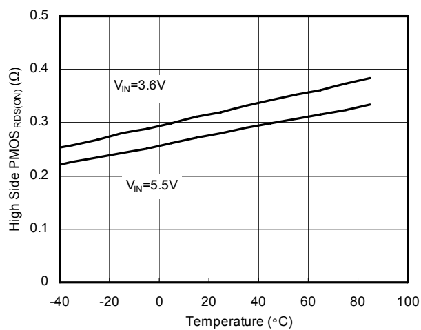
High Side PMOS R_{DS(ON)} vs Temperature
