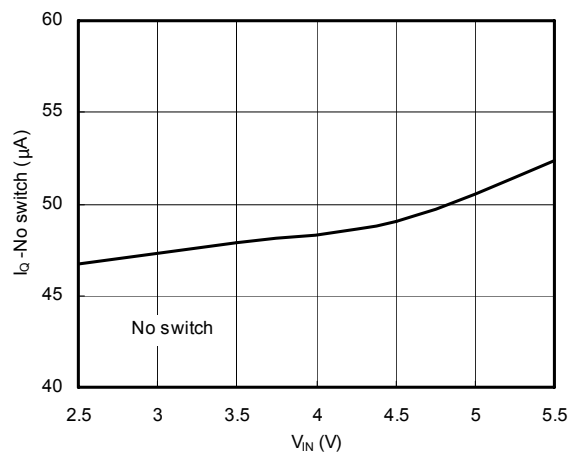
I_Q -No switch vs. V_{IN}
