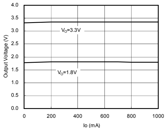
Output Voltage vs. I O
