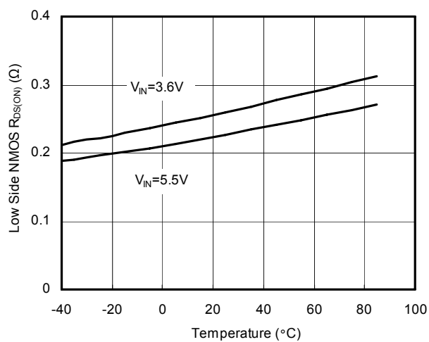
Low Side NMOS R_{DS(ON)} vs Temperature
