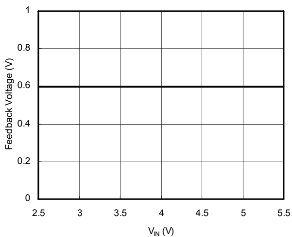
Feedback Voltage vs V_{IN}
