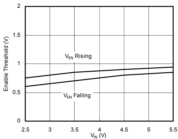
Enable Threshold vs. V_{IN}
