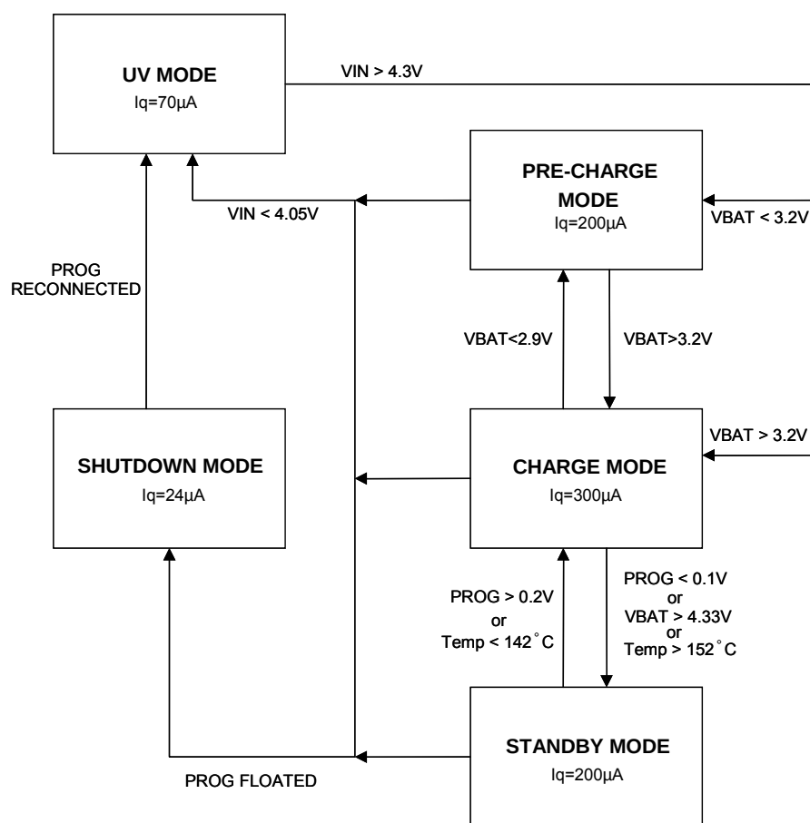
Fig. 1 State Diagram
