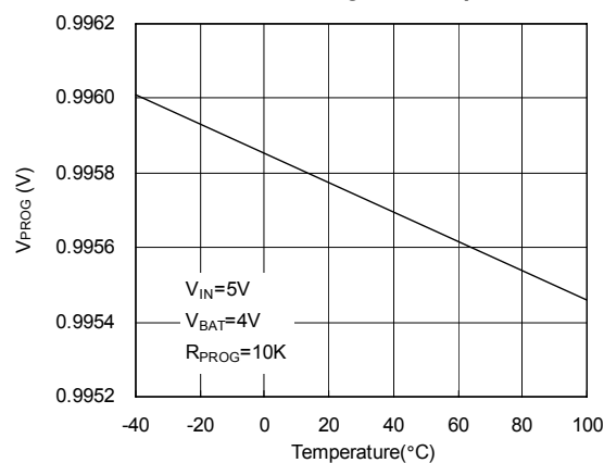
PROG Pin Voltage vs Temperature
