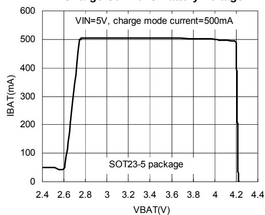
Charge Current vs Battery Voltage
