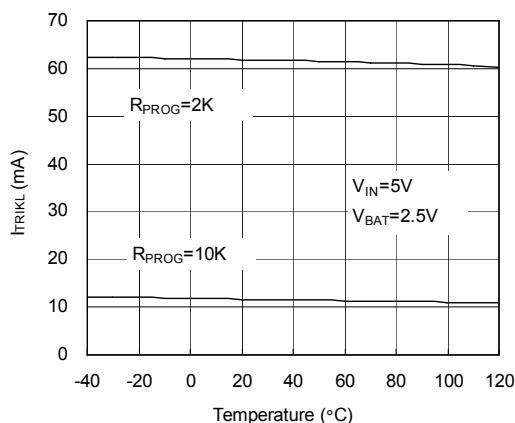
Trickle Charge Current vs Temperature
