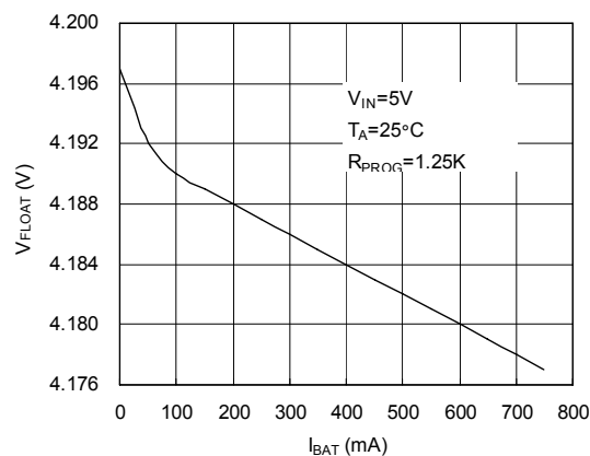
Regulated Output (Float) voltage vs Charge Current
