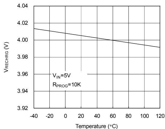
Recharge Voltage Threshold vs Temperature
