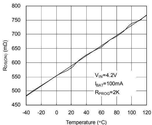
Power FET "ON" Resistance vs Temperature
