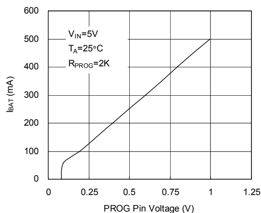
Charge Current vs PROG Pin Voltage
