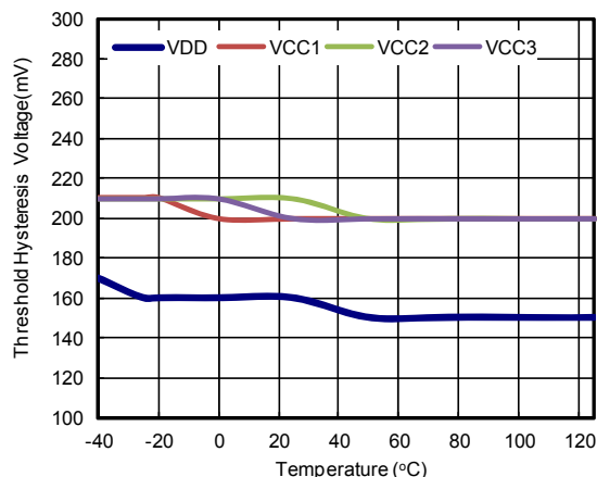
VTH Hysteresis Voltage vs. Temperature
