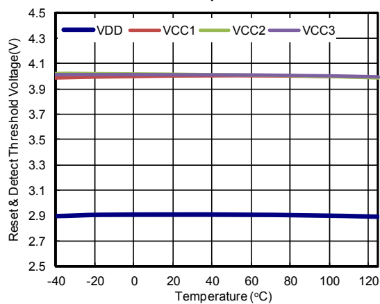
Reset & Detect Threshold Voltage vs. Temperature
