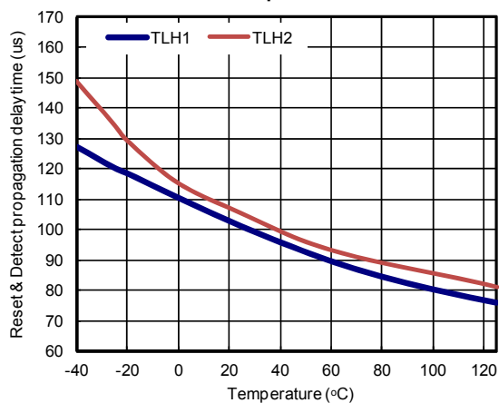
Reset & Detect propagation delay time vs. Temperature
