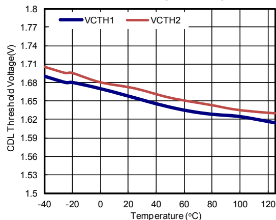
CDL Threshold Voltage vs. Temperature
