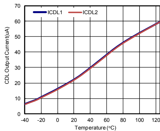
CDL Output Current vs. Temperature
