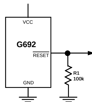
Figure2. RESET Valid to V_{CC} = Ground Circuit
