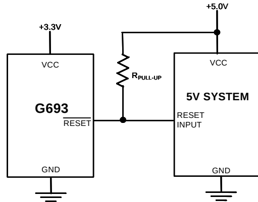
Figure4. G693L Open-Drain \overline{RESET} Output Allows Use with Multiple Supplies
