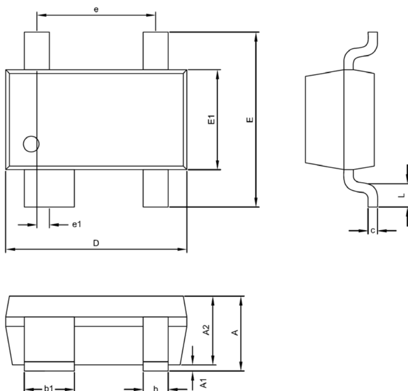
SOT-143 (TC) Package
