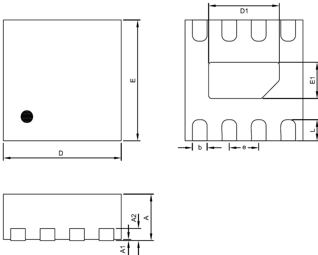
TDFN2X2-8 (RC) Package
