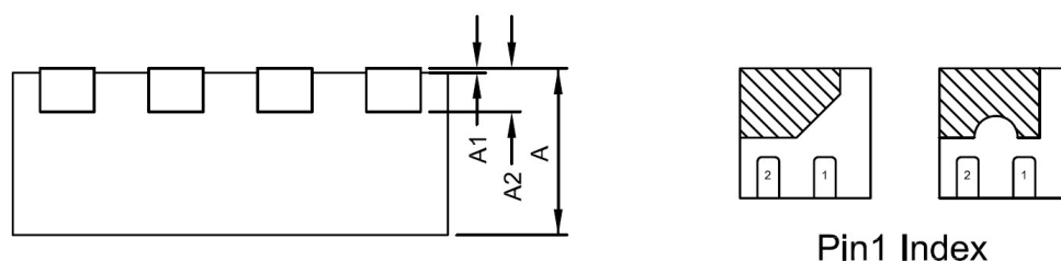
TDFN2X2-8 Package
