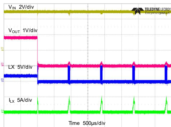
Short Circuit waveform V_{OUT}=1.8V
