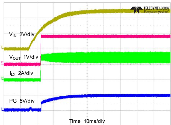
Start-up Through VIN V_{OUT}=1.8V , I_{OUT}=3A
