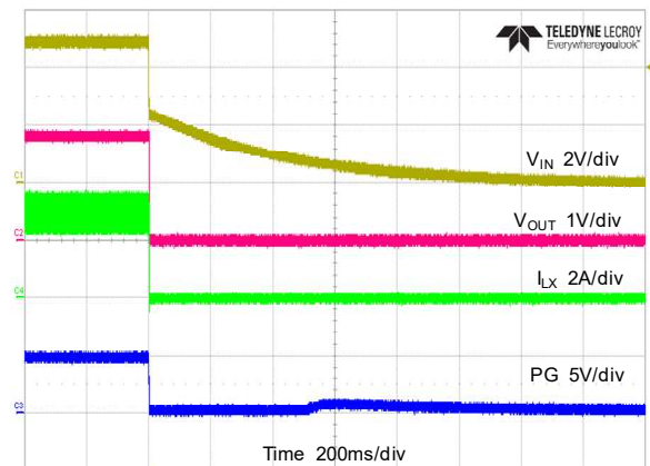
Start-down Through VIN V_{OUT}=1.8V , I_{OUT}=3A
