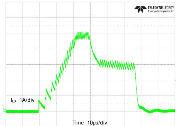
Current Limit
