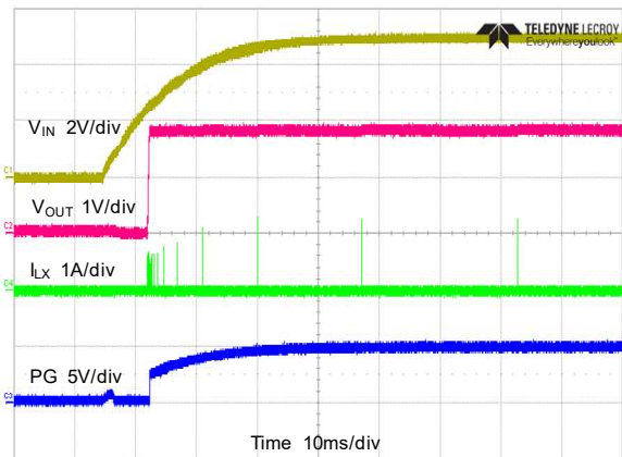
Start-up Through VIN V_{OUT}=1.8V , No Load
