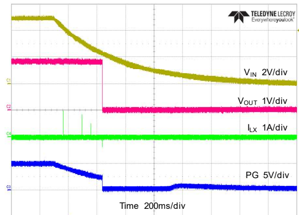
Start-down Through VIN V_{OUT}=1.8V , No Load
