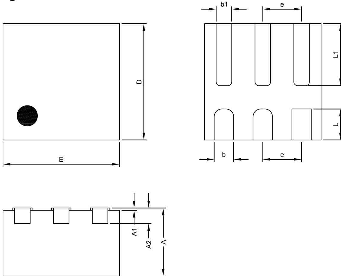
ADFN1.5X1.5-6 Package
