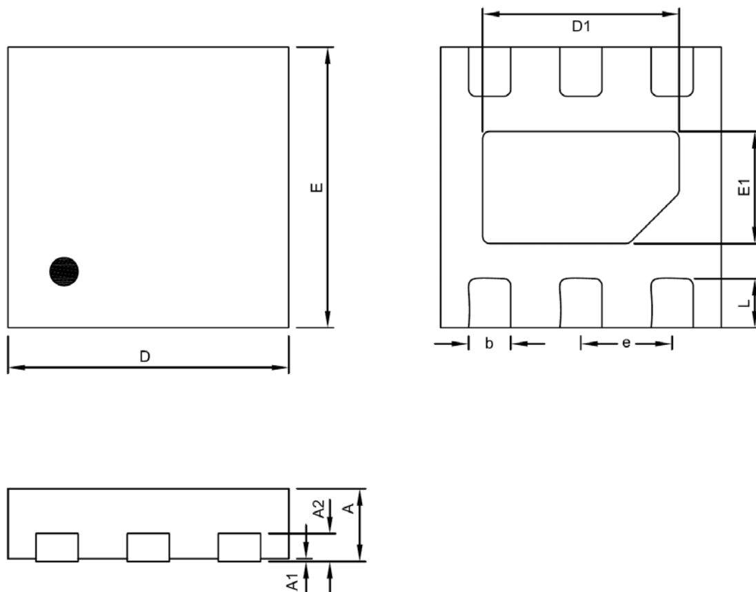
WDFN2X2-6 Package
